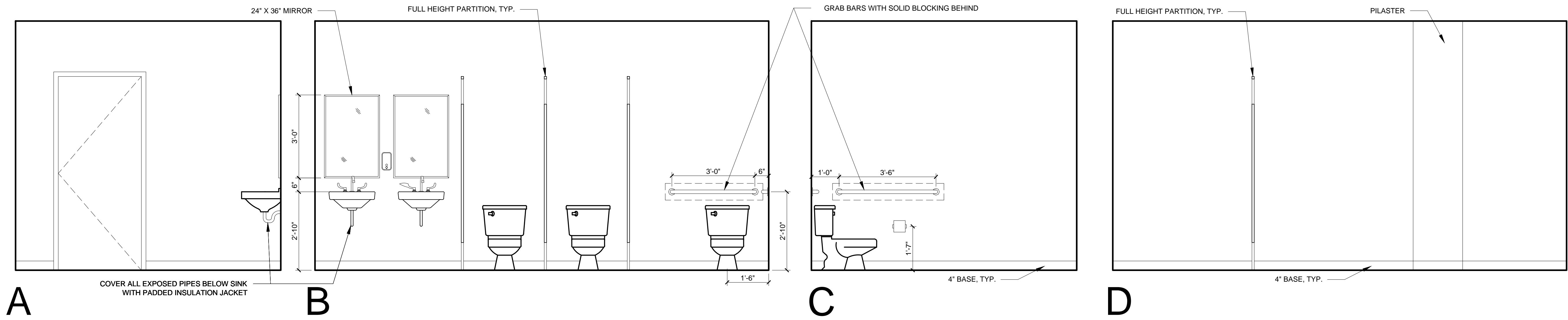
1 WOMEN'S BATHROOM 112 1/2" = 1'-0"
