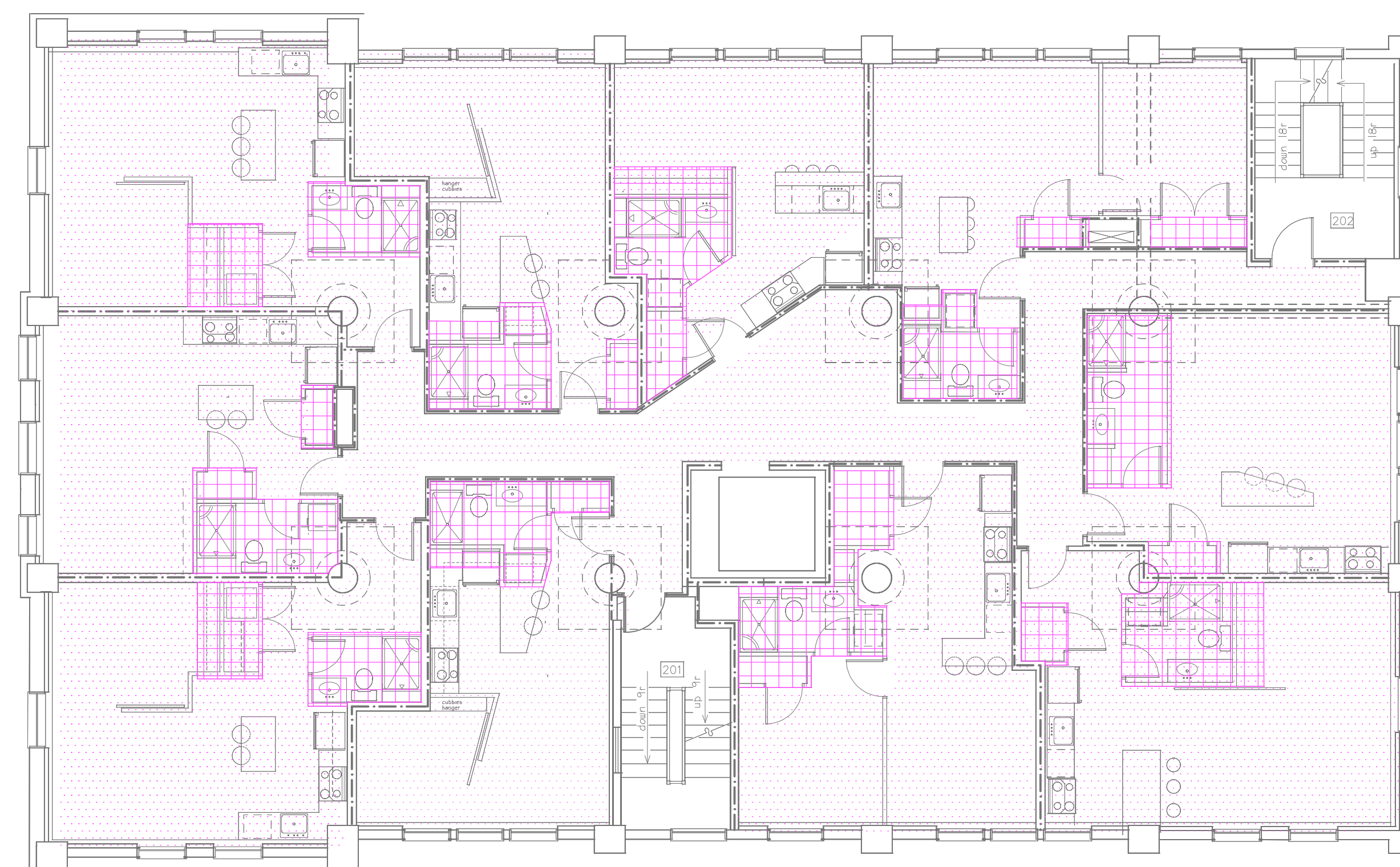
2nd, 3rd, 4th floors duct ceiling plan
