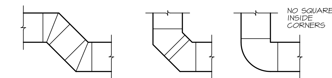
3 UNACCEPTABLE DUCT FITTINGS NO SCALE THESE TYPES OF FITTINGS PROHIBITED UNLESS SPECIFICALLY INDICATED OTHERWISE ELBOWS TO BE SMOOTH, LONG RADIUS ONLY SEGMENTED ELBOWS ARE PROHIBITED
