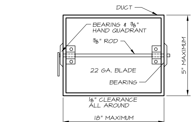
4 SHOP FABRICATED MANUAL DAMPER NO SCALE
