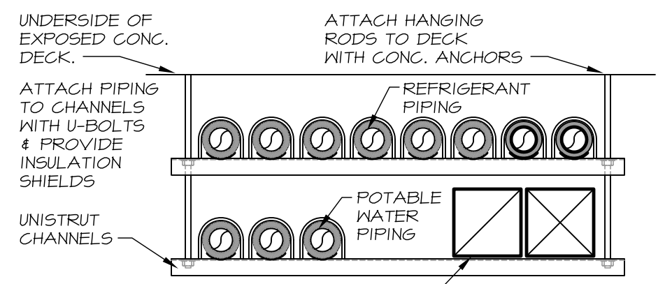
1 TYPICAL DUCT & PIPING SUPPORT RACK NO SCALE
