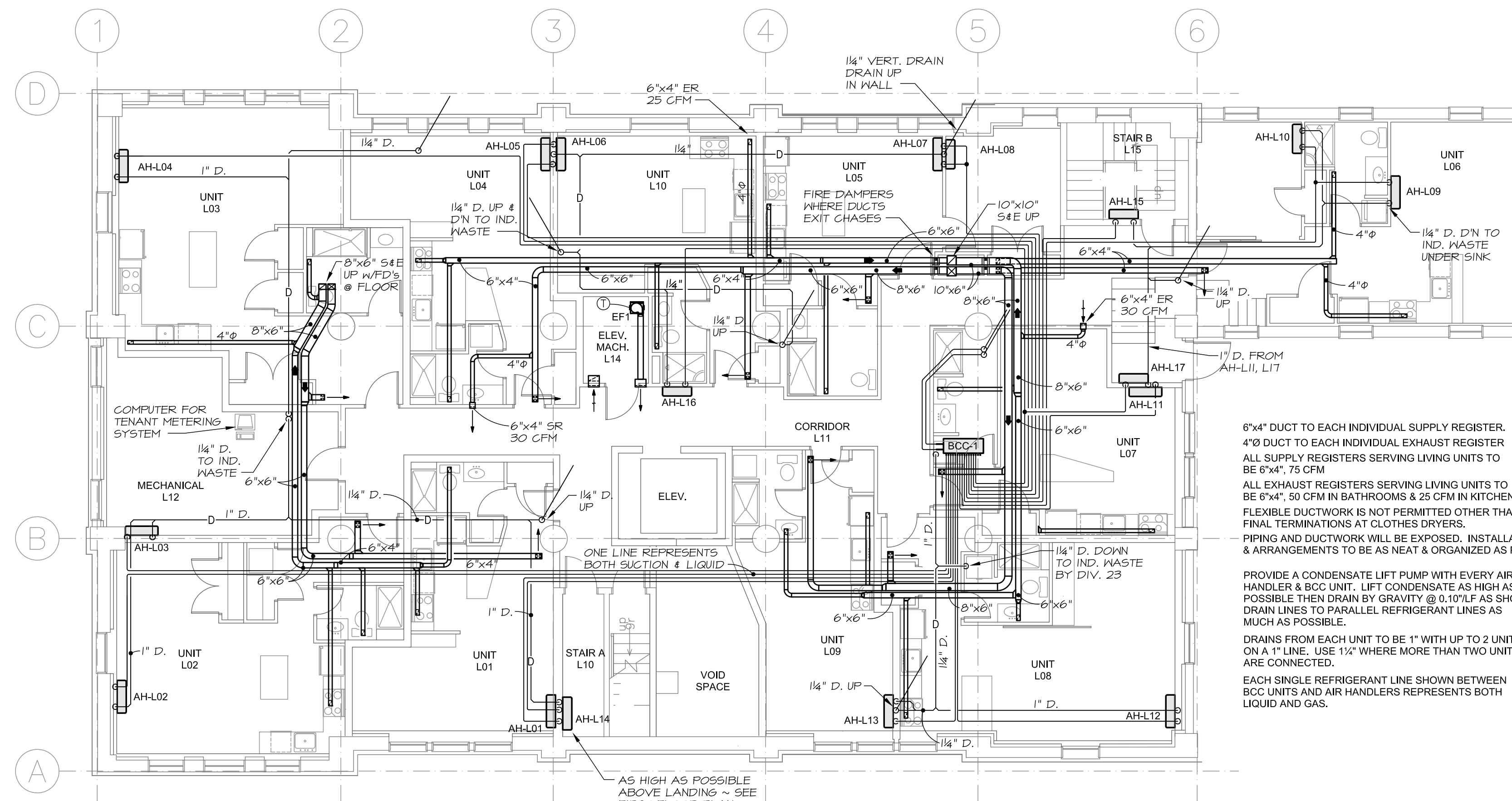
6 LOWER LEVEL PLAN SCALE: 1/8" = 1'-0" ELEV. 07.55'
