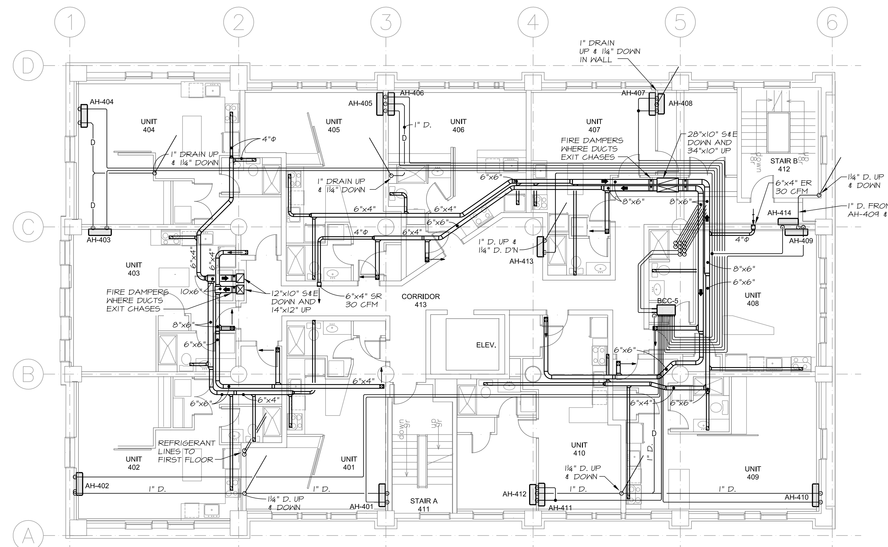
2 FOURTH FLOOR PLAN SCALE: 1/8" = 1'-0" ELEV. 53.05'
