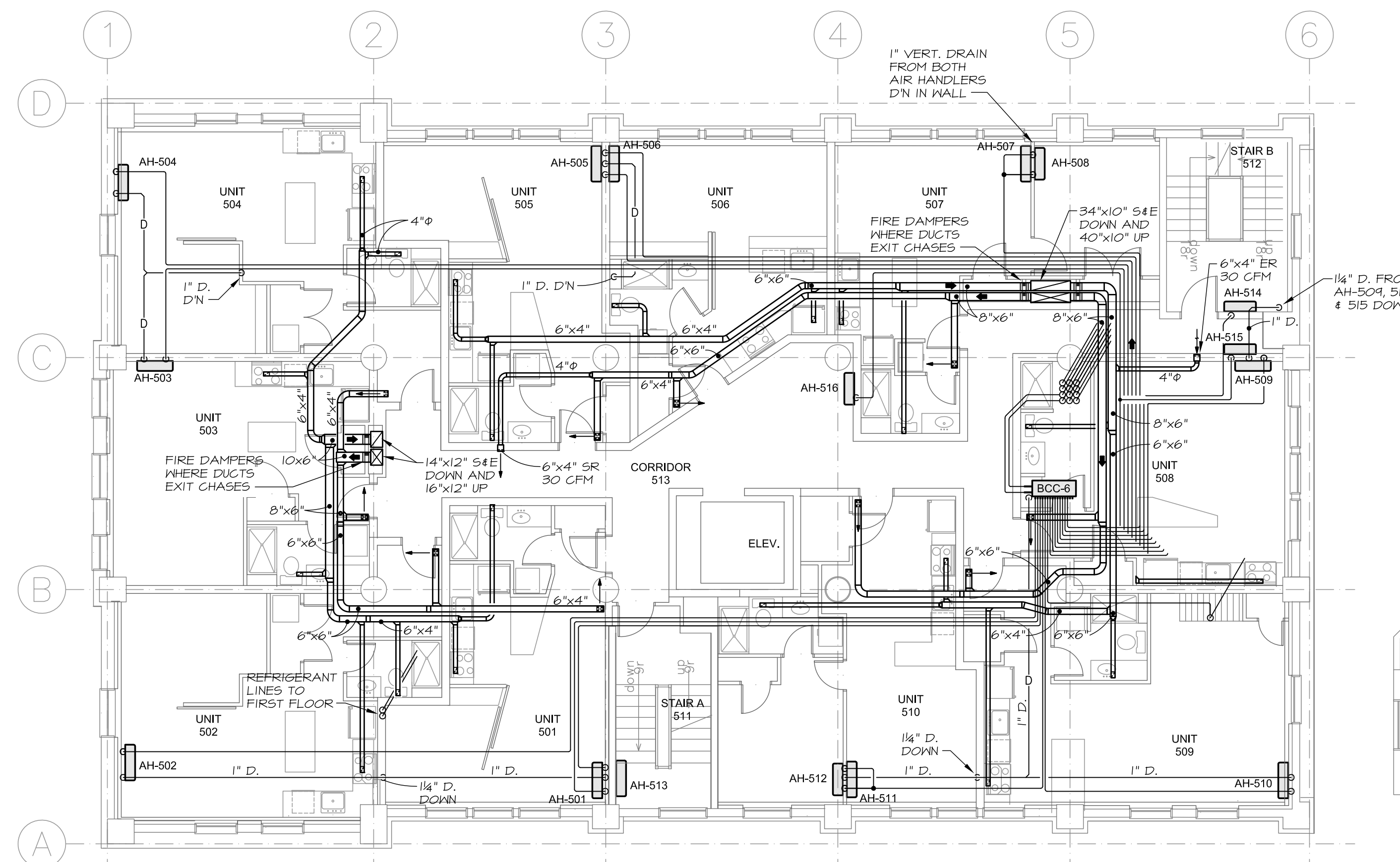
1 FIFTH FLOOR PLAN SCALE: 1/8" = 1'-0" ELEV. 64.55'
