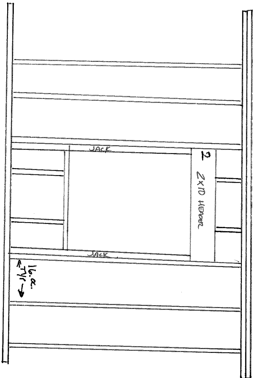
TYP. WALL SECTION
