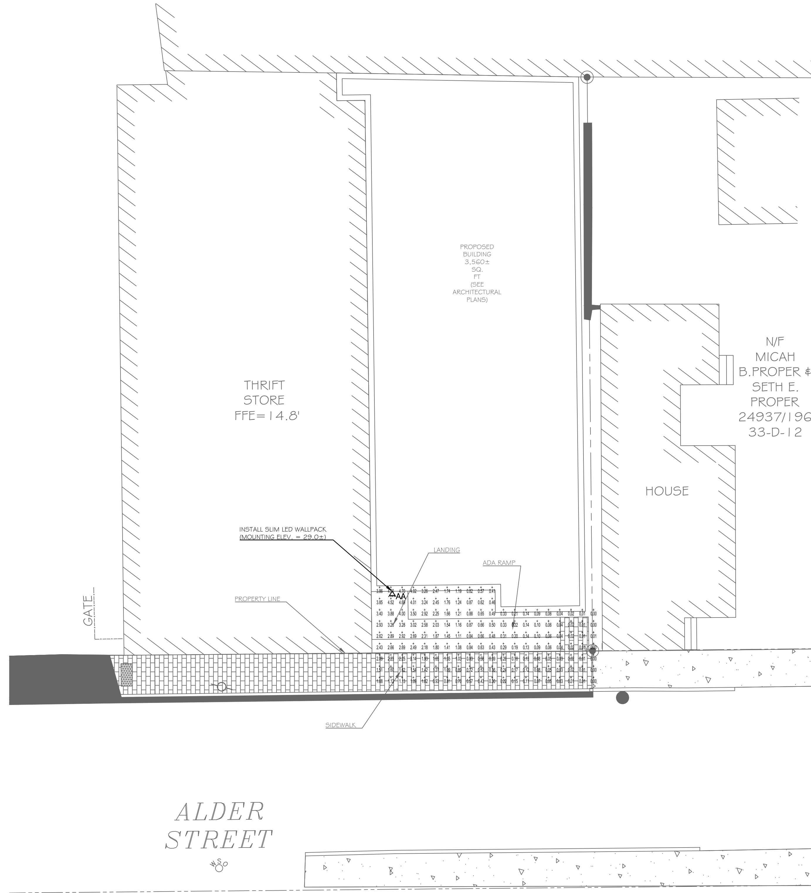
1 EXTERIOR LIGHTING SCALE: 1"=10'
