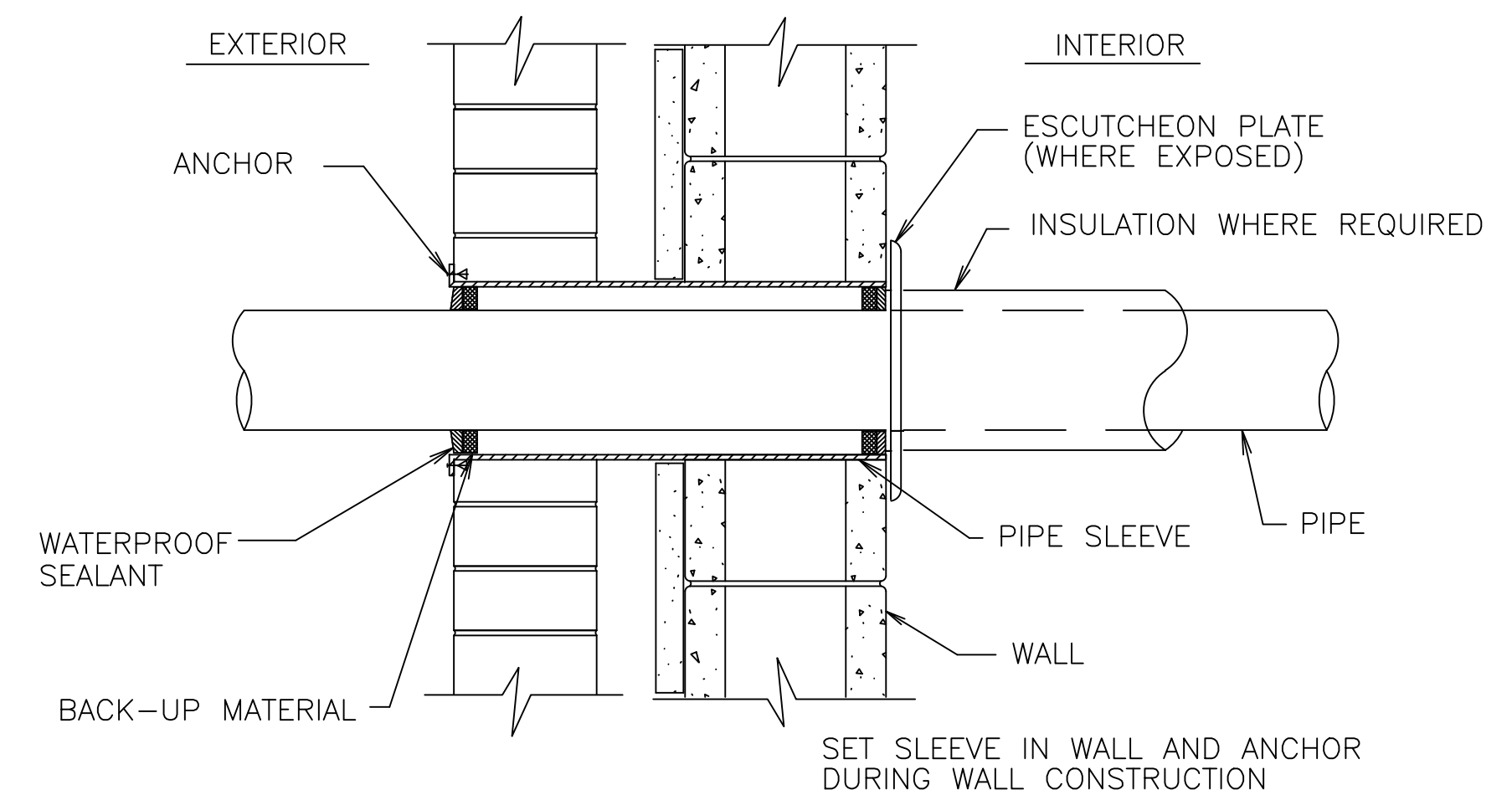
PIPE SLEEVE THRU EXTERIOR WALL 1 NO SCALE
