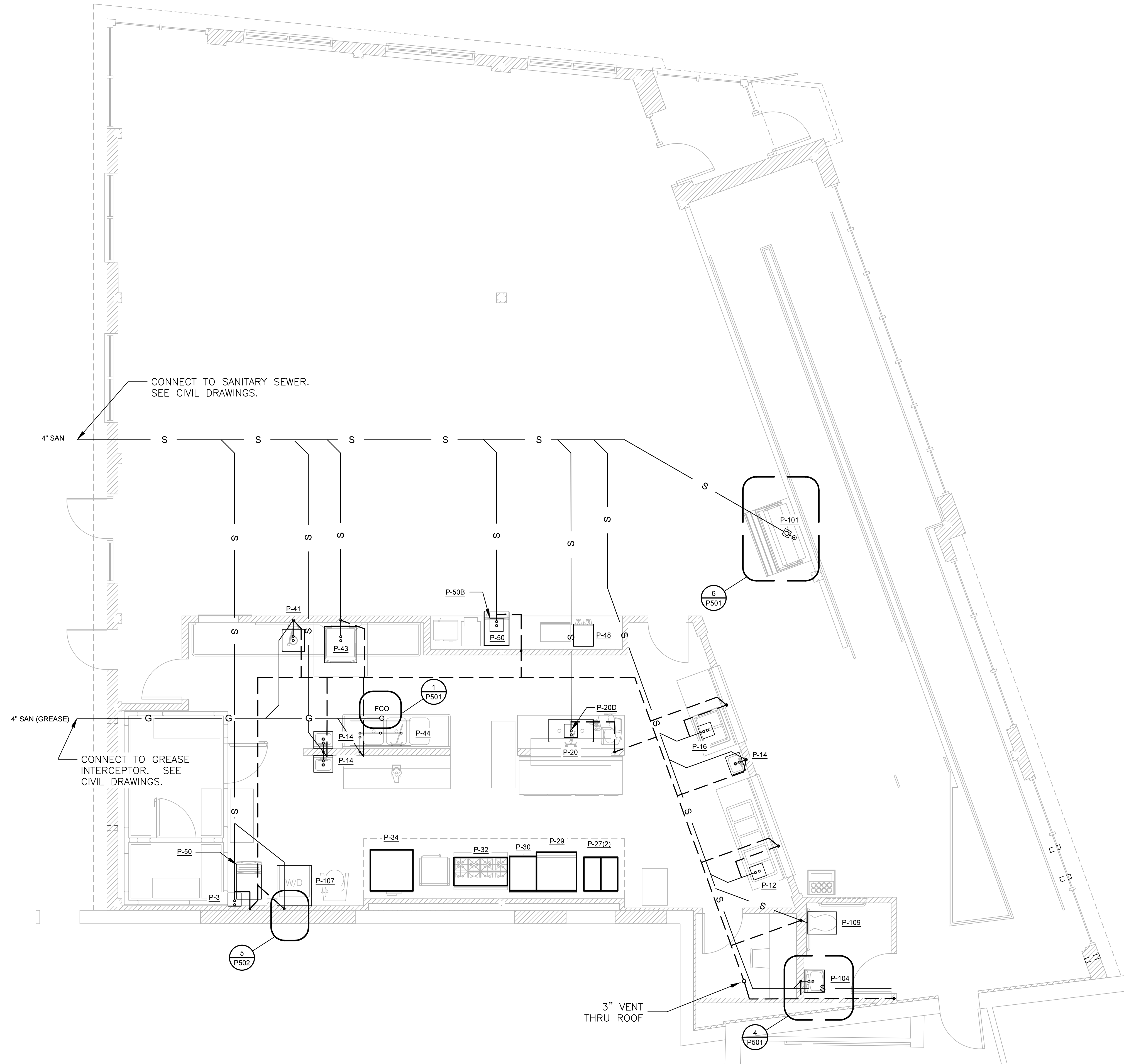
1 DINING HALL PLUMBING DWV PLAN 1/8" = 1'0"
