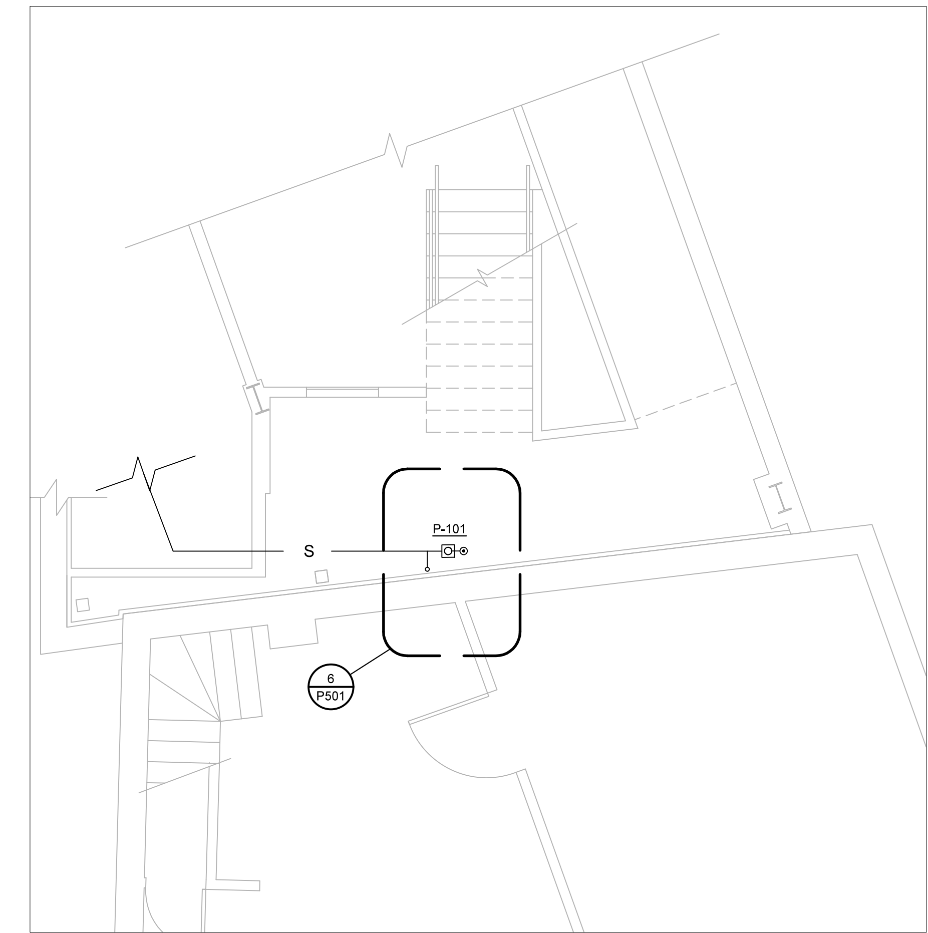
2 DINING HALL UNDER RAMP PLUMBING DWV PLAN 1/8" = 1'0"
