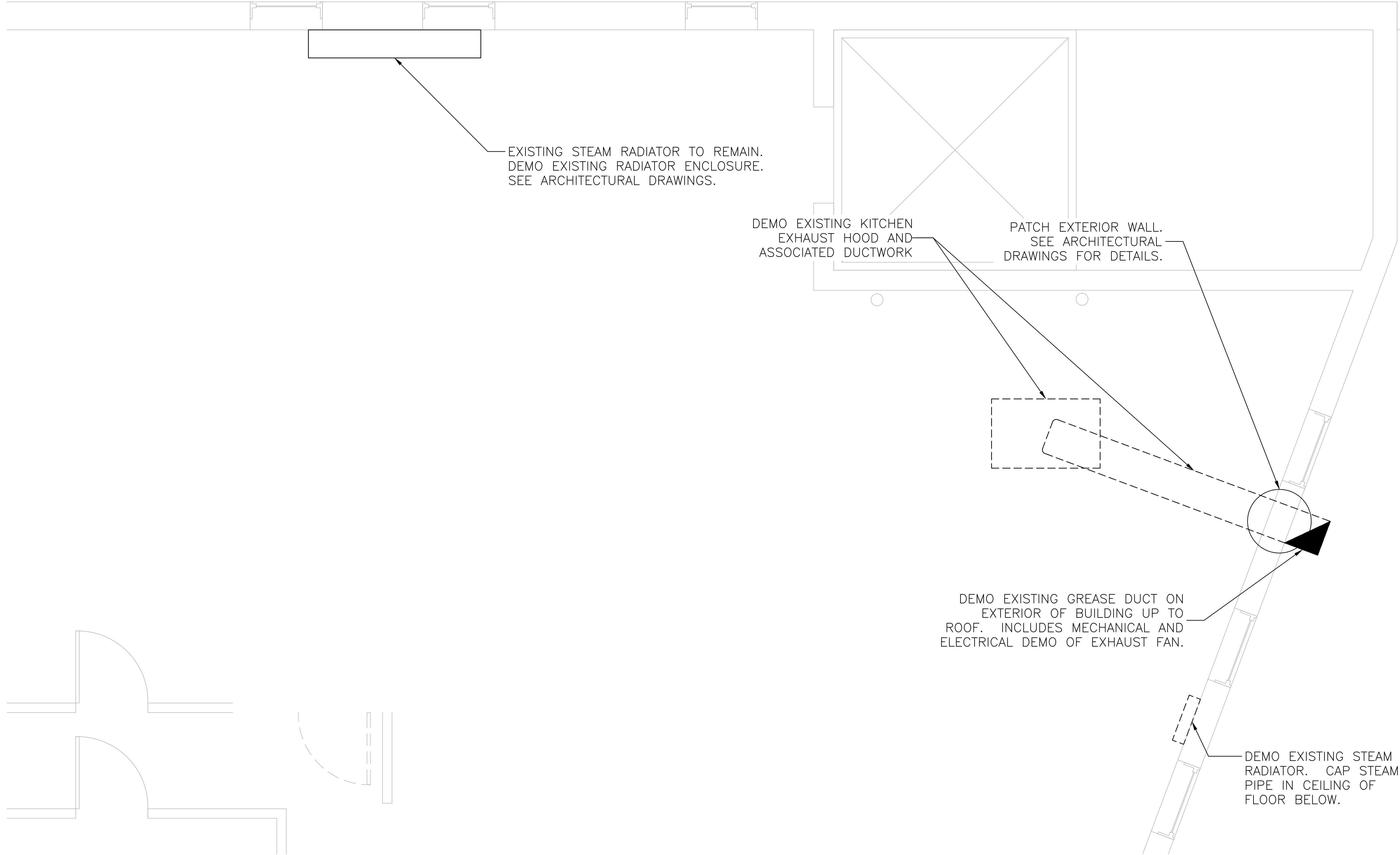
1 APARTMENT AND COMMUNITY ROOM HVAC DEMO PLAN 1/2" = 1'0"
