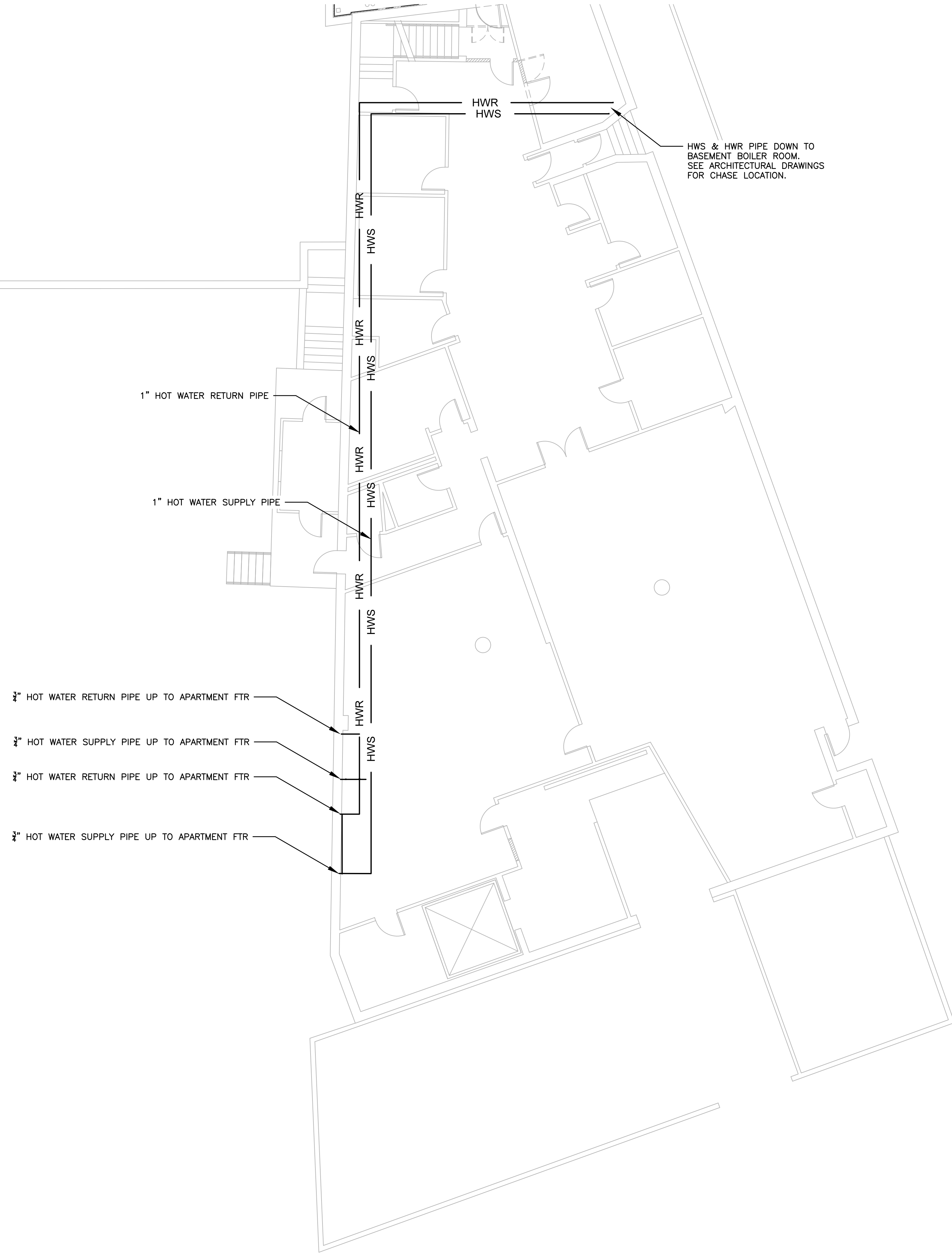
1 APARTMENT FIRST FLOOR HVAC PLAN 1/8" = 1'-0"
