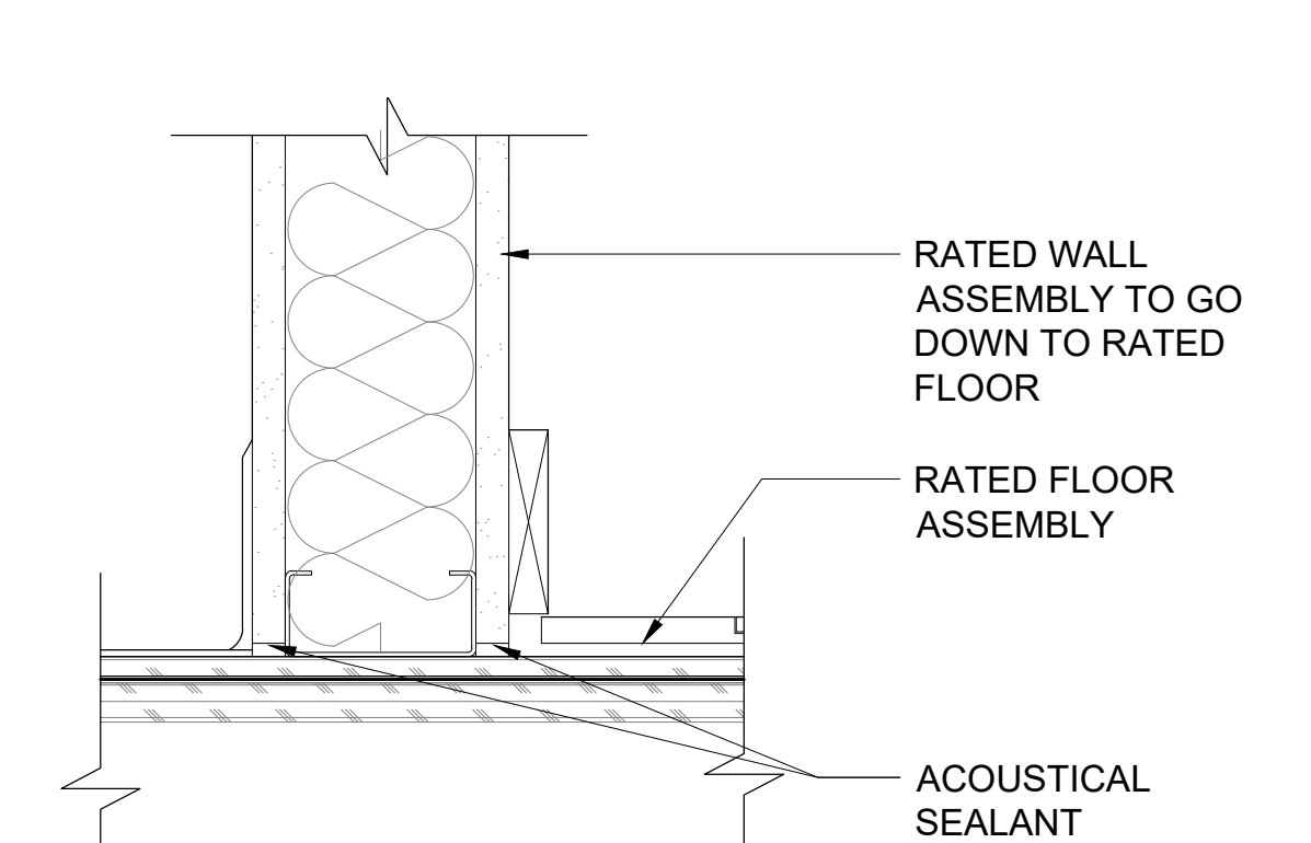
9 BOTTOM OF RATED WALL SCALE: 3" = 1'-0"
