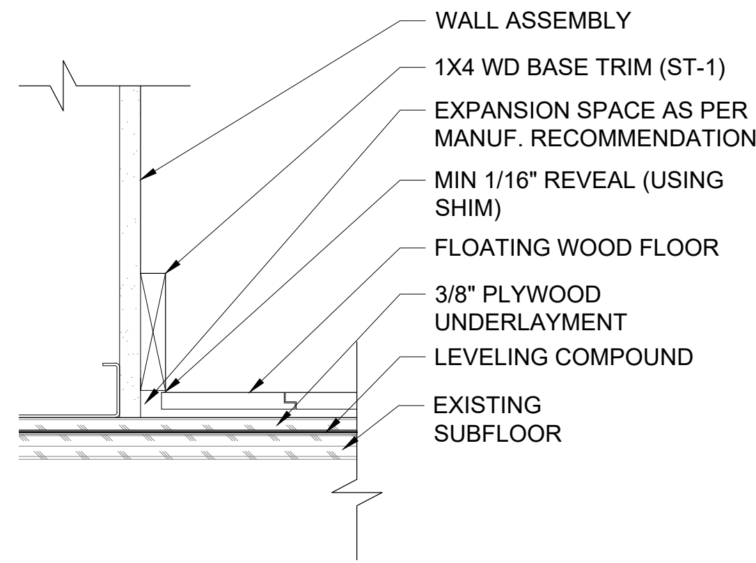
1 WOOD BASE/FLOOR DETAIL SCALE: 3" = 1'-0"
