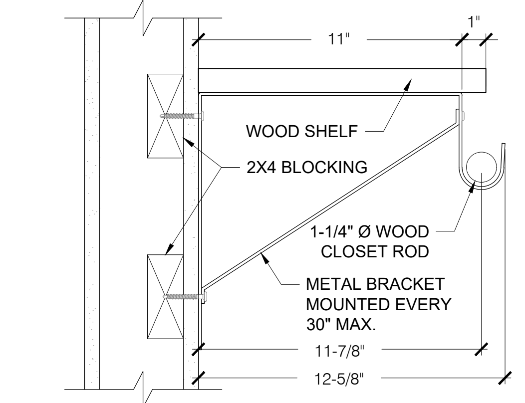
5 POLE & SHELF DETAIL SCALE: 3" = 1'-0"
