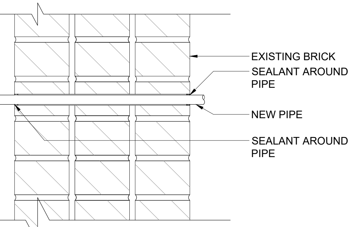
11 PIPE PENETRATION @ BRICK SCALE: 3" = 1'-0"
