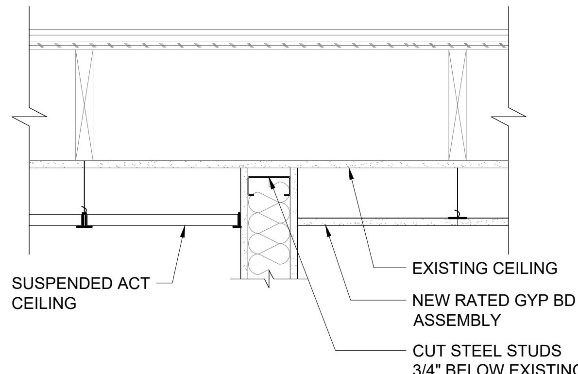
8 TOP OF RATED WALL SCALE: 1-1/2" = 1'-0"
