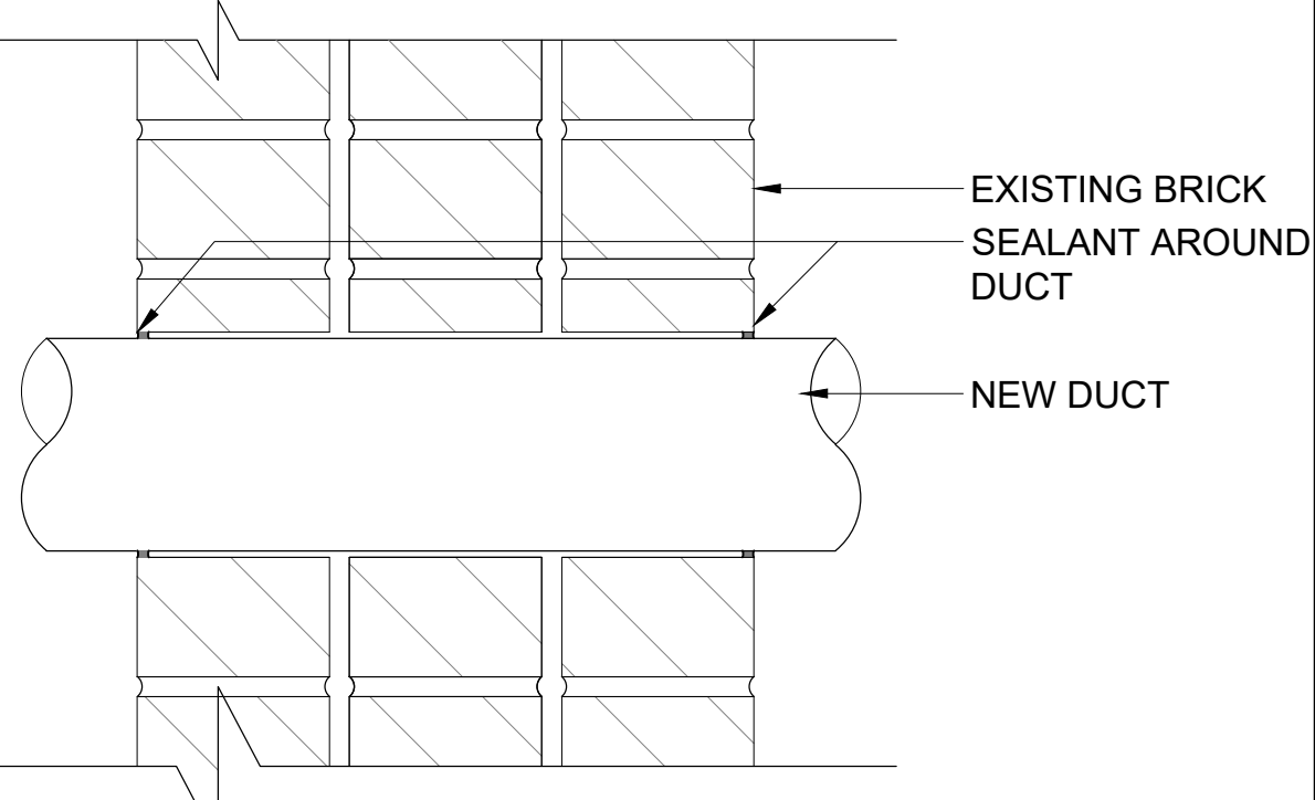
12 DUCT HOOD @ BRICK SCALE: 3" = 1'-0"
