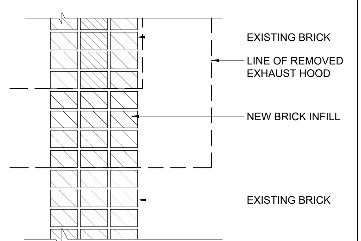
10 EXHAUST HOOD BRICK INFILL SCALE: 3/8" = 1'-0"
