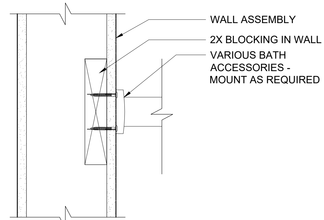
6 BATH ACCESSORY MNTING SCALE: 1/2" = 1'-0"
