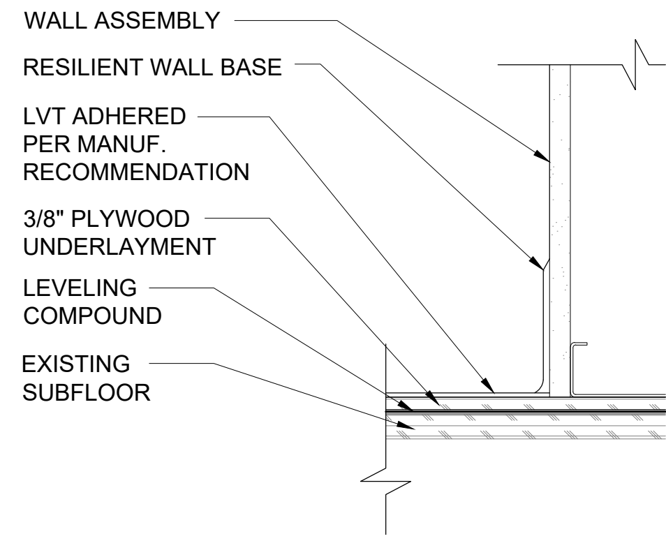
2 RWB/FLOOR DETAIL SCALE: 3" = 1'-0"
