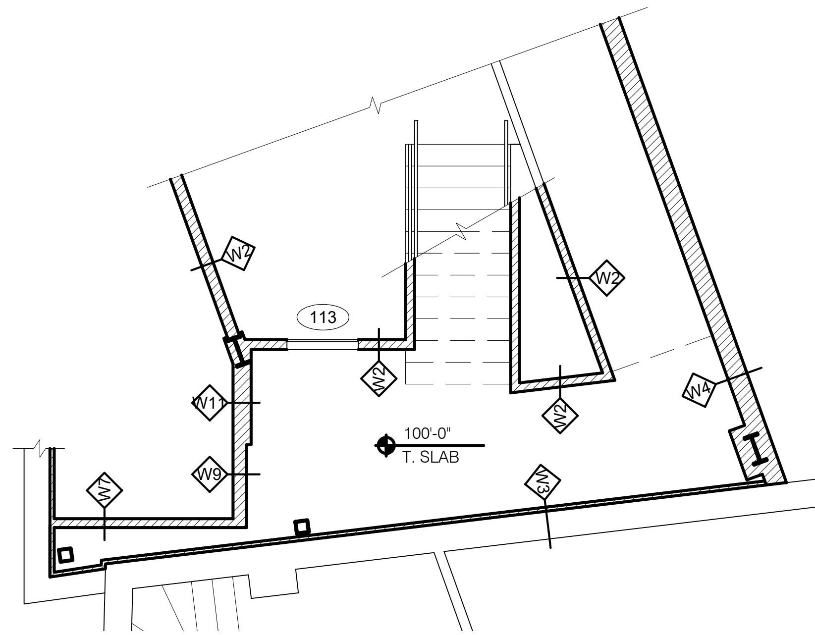
1 UNDER RAMP PLAN SCALE: 1/4" = 1'-0"
