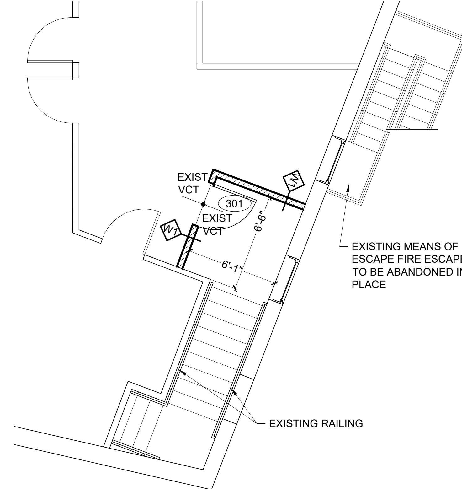
4 THIRD FLOOR EGRESS STAIR SCALE: 1/4" = 1'-0"
