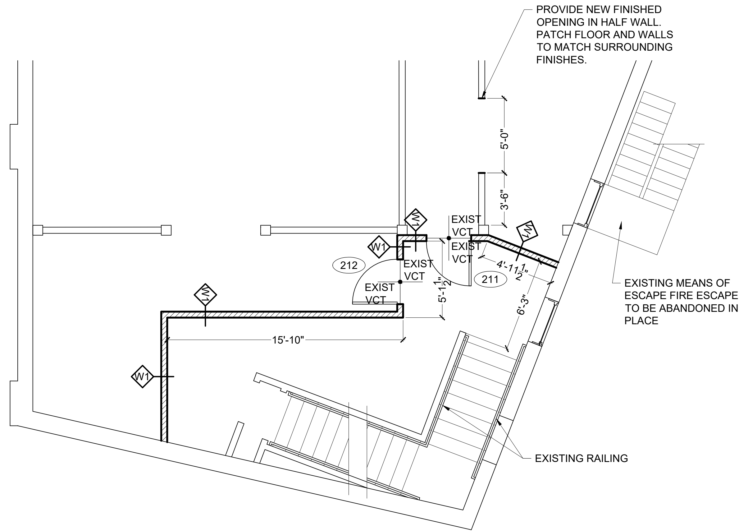
3 SECOND FLOOR EGRESS STAIR SCALE: 1/4" = 1'-0"
