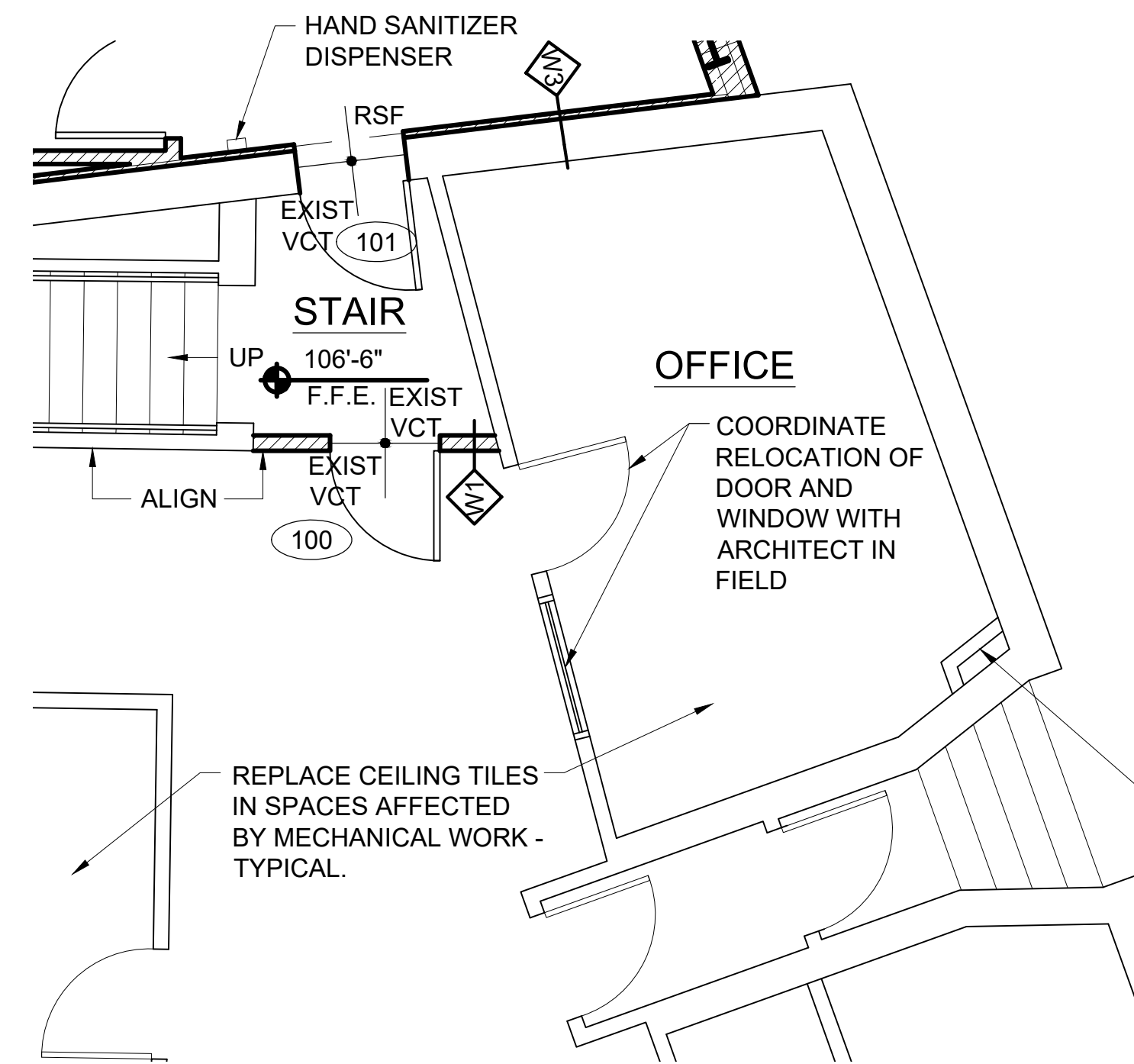
2 DINING HALL PLAN - CONT. SCALE: 1/4" = 1'-0"
