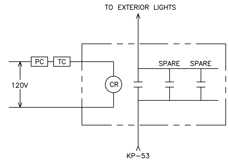
③ EXTERIOR LIGHTING CONTROL
