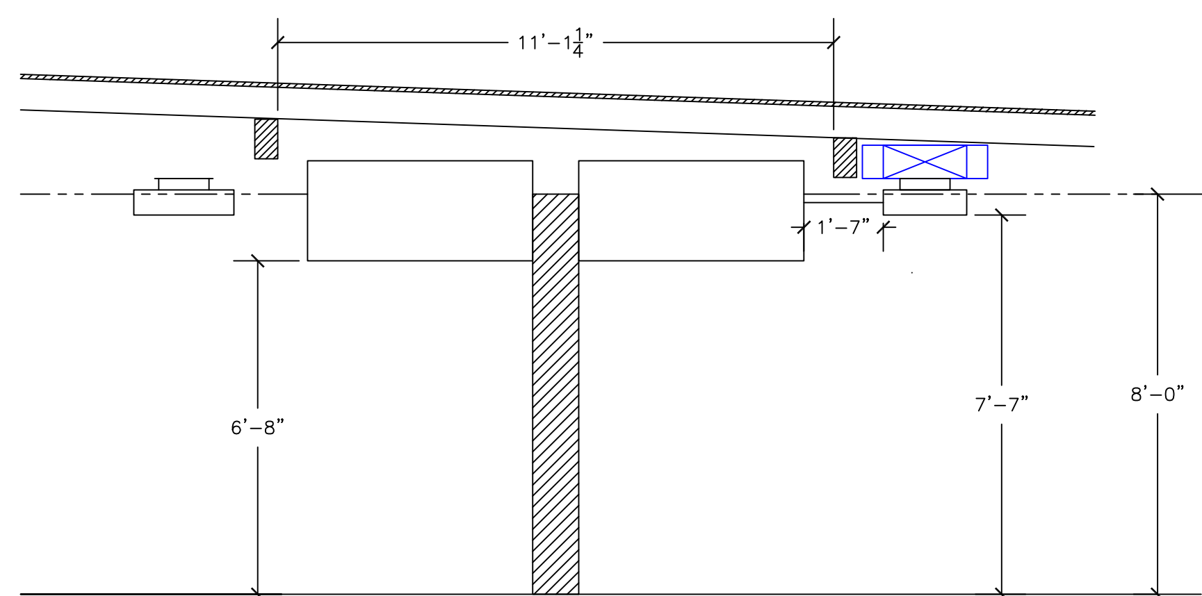
ELEVATION AT HOODS \frac{3}{8}''=1'-0''
