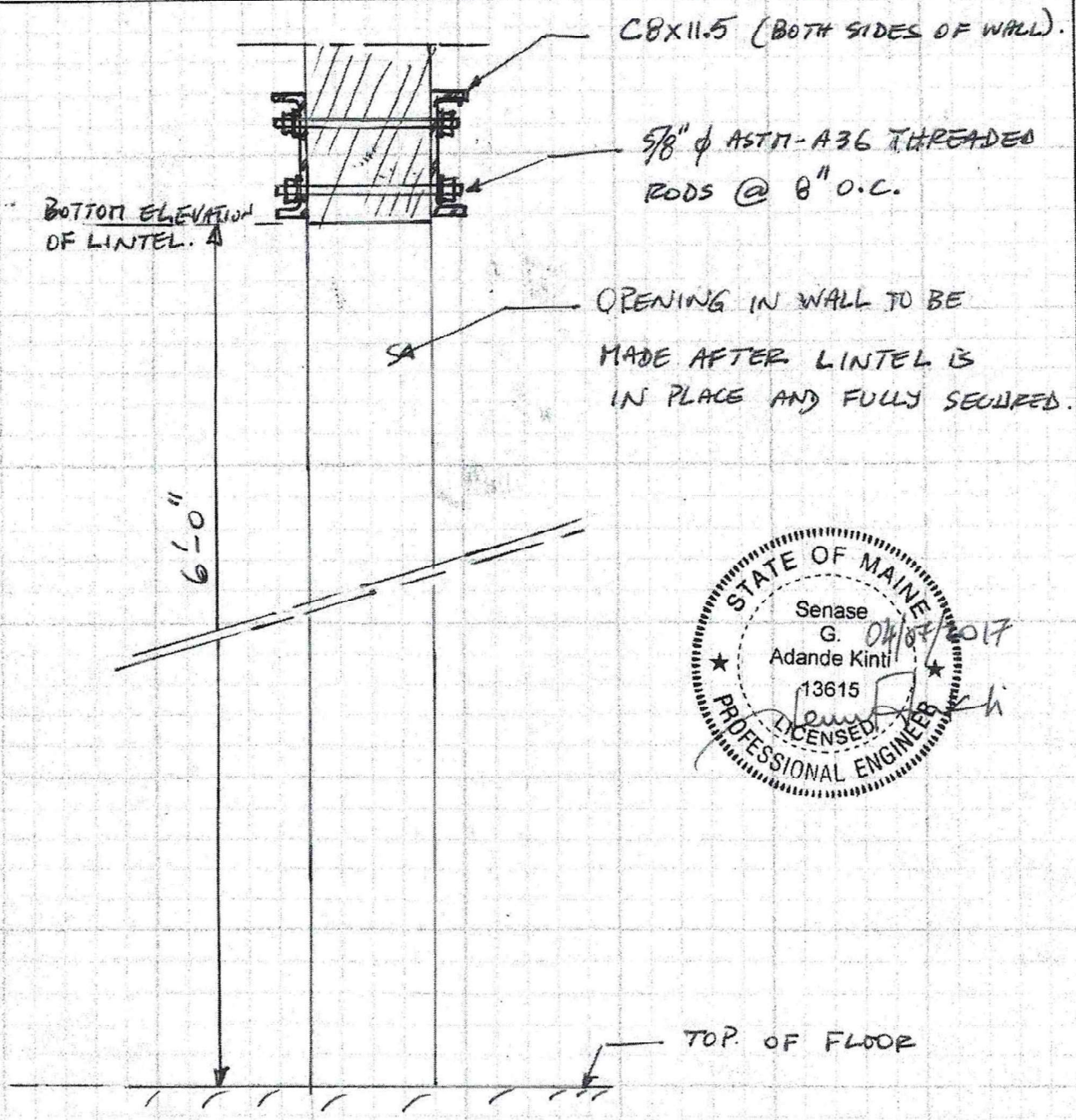
EXISTING WALL OPENING FRAMING - SECTION A (N.T.S.) SK-01
