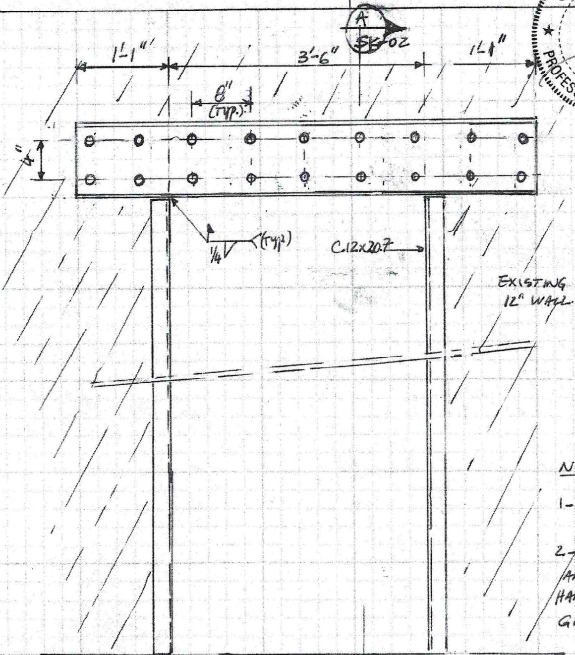
EXISTING WALL OPENING FRAMING. ELEVATION (N.T.S.)
