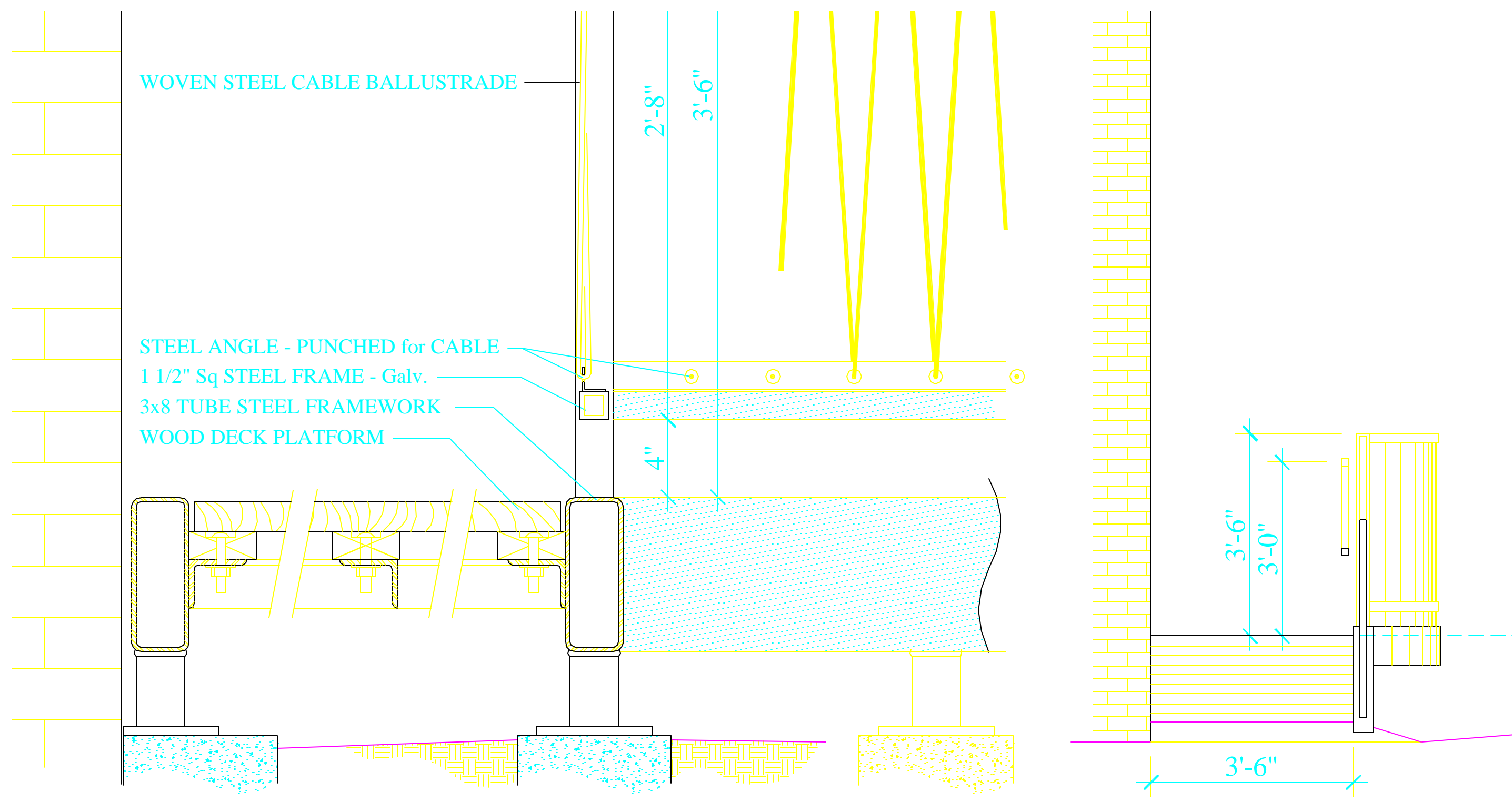
RAMP - DTL SECTION
