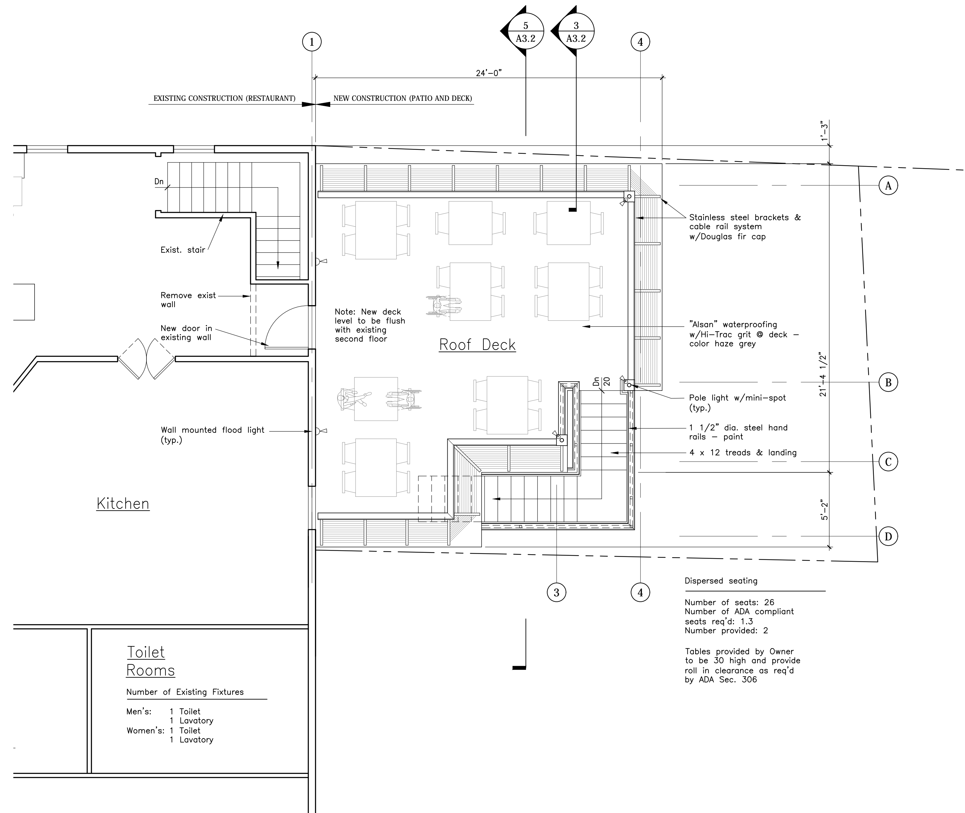
2 Proposed Second Floor Plan
