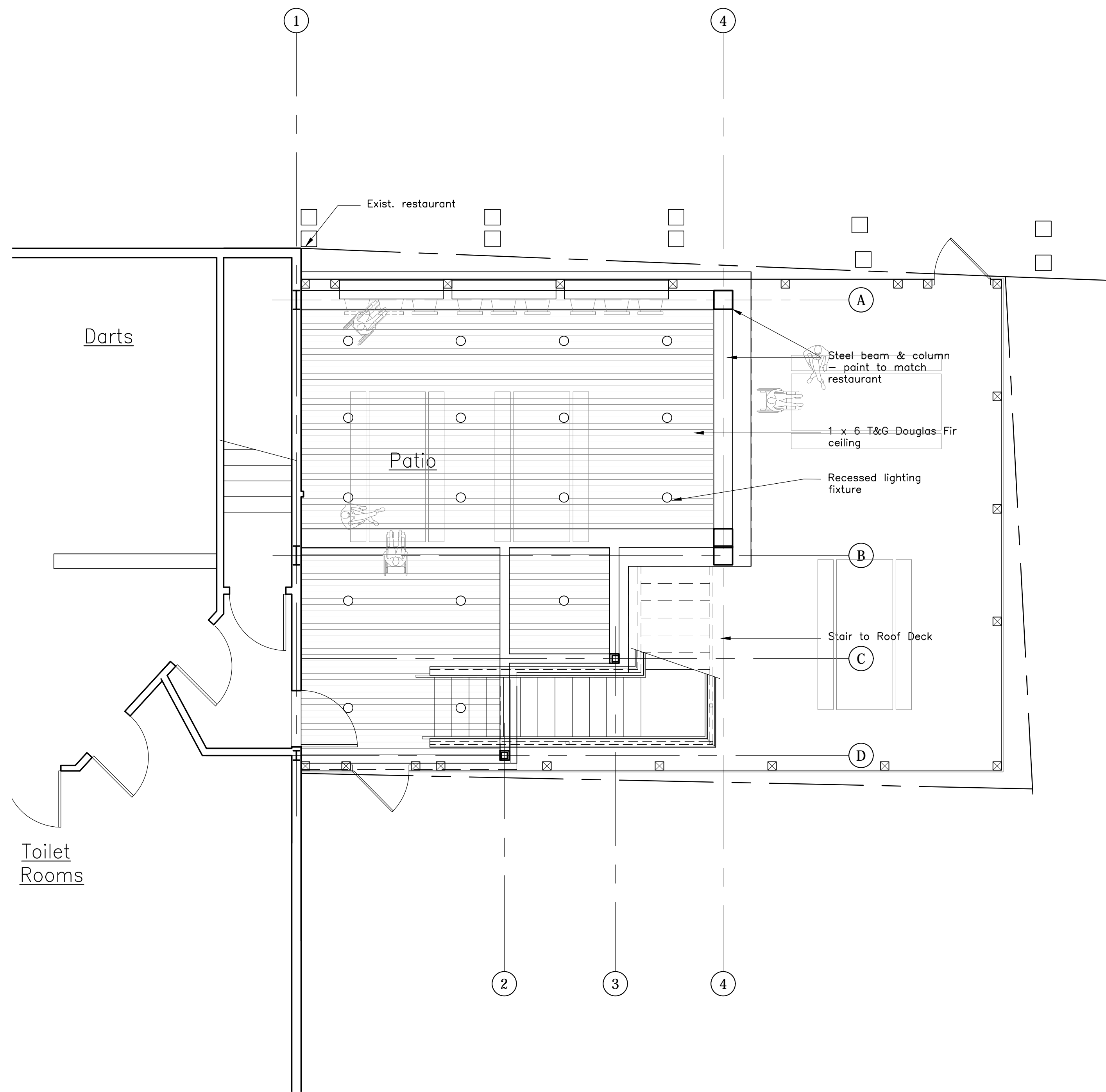
3 First Floor Lighting Plan
