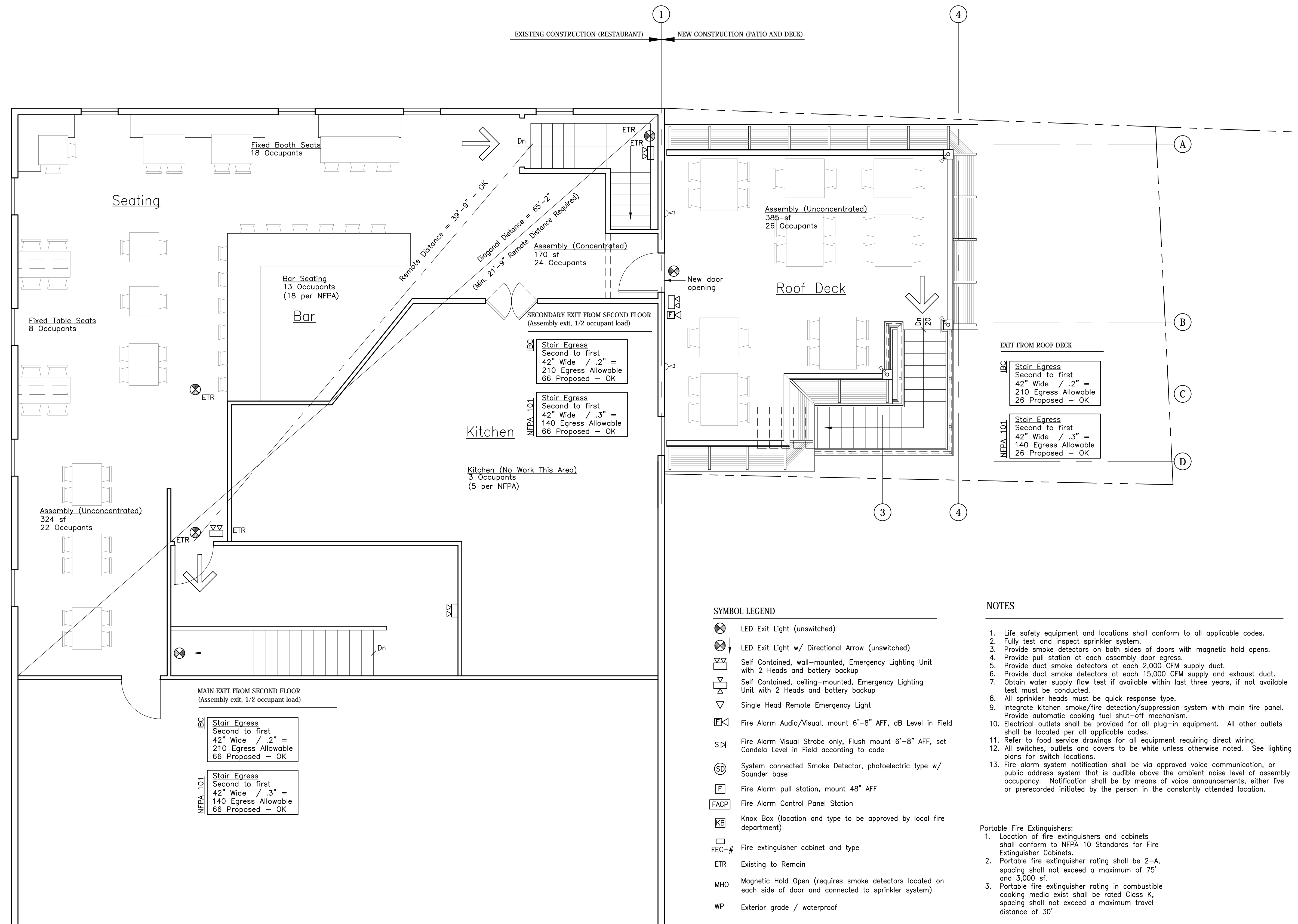
1 Second Floor Code Review Plan
