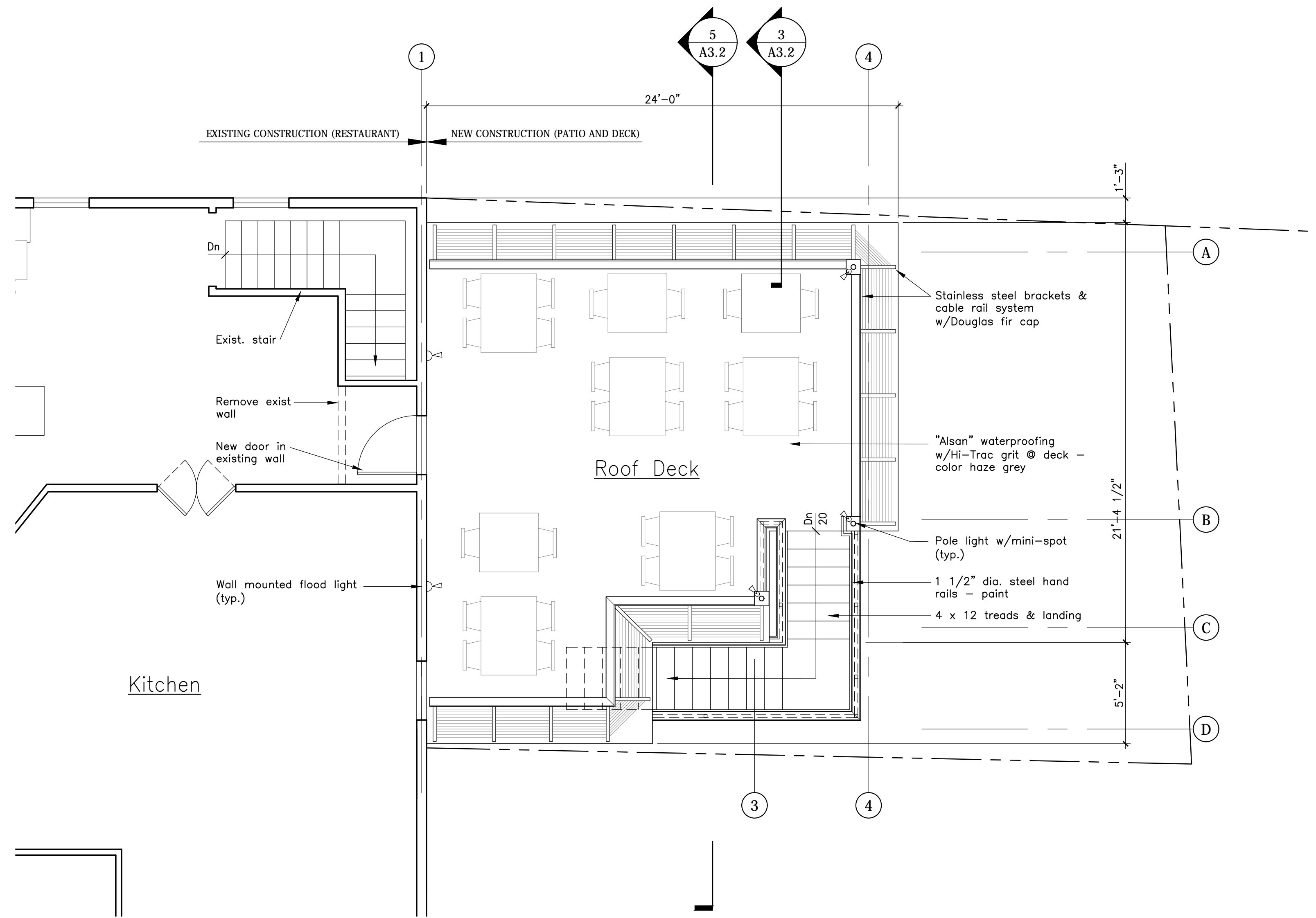
2 Proposed Second Floor Plan Scale: 1/4" = 1'-0"
