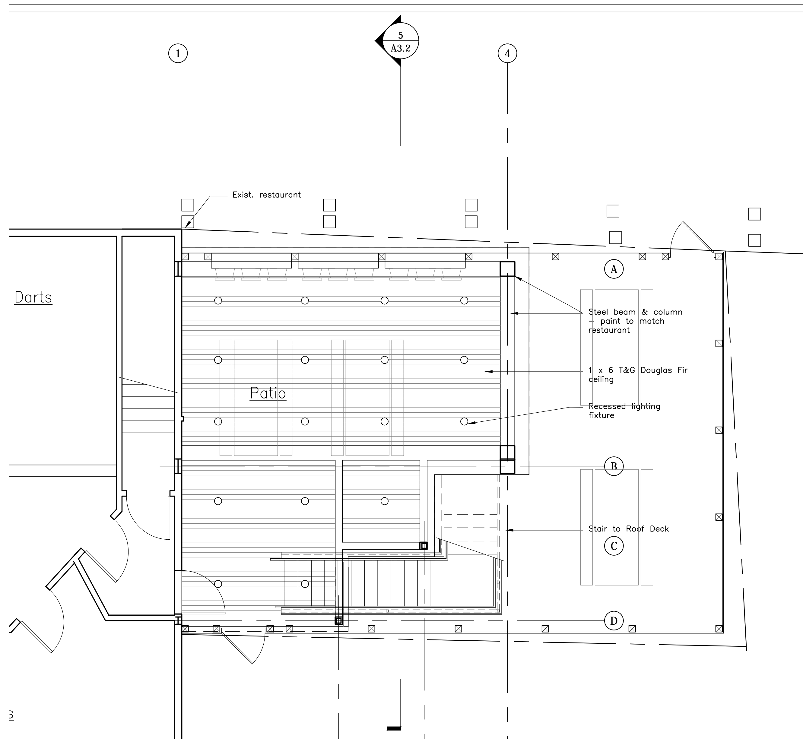
3 First Floor Lighting Plan Scale: 1/4" = 1'-0"
