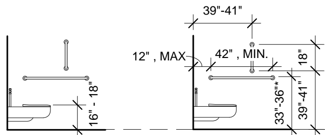
FIG. 604.4 HEIGHT TO TOP OF SEAT
