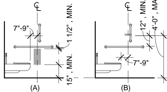
FIG. 604.7 DISPENSER LOCATION (A) BELOW GRAB BAR (B) ABOVE GRAB BAR
