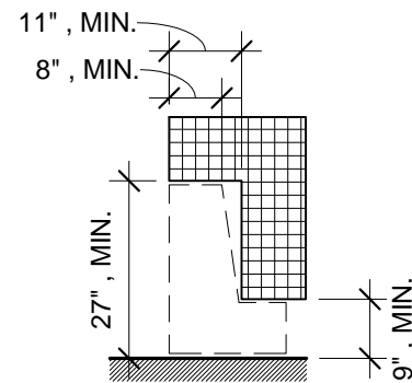
FIG. 306.3 - KNEE CLEARANCE
