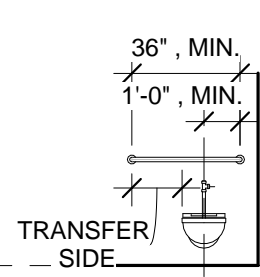
FIG. 604.5.2 REAR WALL GRAB BAR FOR WATER CLOSET
