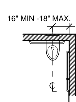
FIG. 604.2 WATER CLOSET LOCATION
