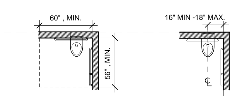
FIG. 604.3.1 SIZE OF CLEARANCE FOR WATER CLOSET
