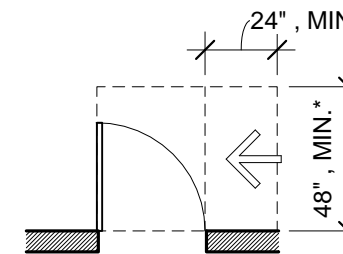
(F) LATCH APPROACH, PULL SIDE
