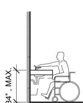
FIG. 606.3 - HEIGHT OF LAVATORIES AND SINKS
