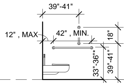
FIG. 604.5.1 SIDE WALL GRAB BAR FOR WATER CLOSET * TO TOP OF GRAB BAR
