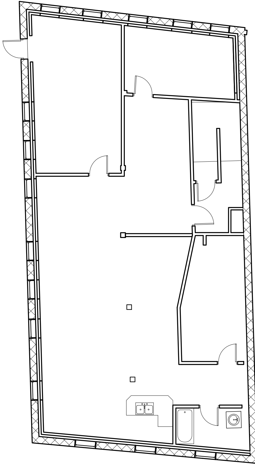
① Level 4 @ 444 Fore 1/8" = 1'-0"
