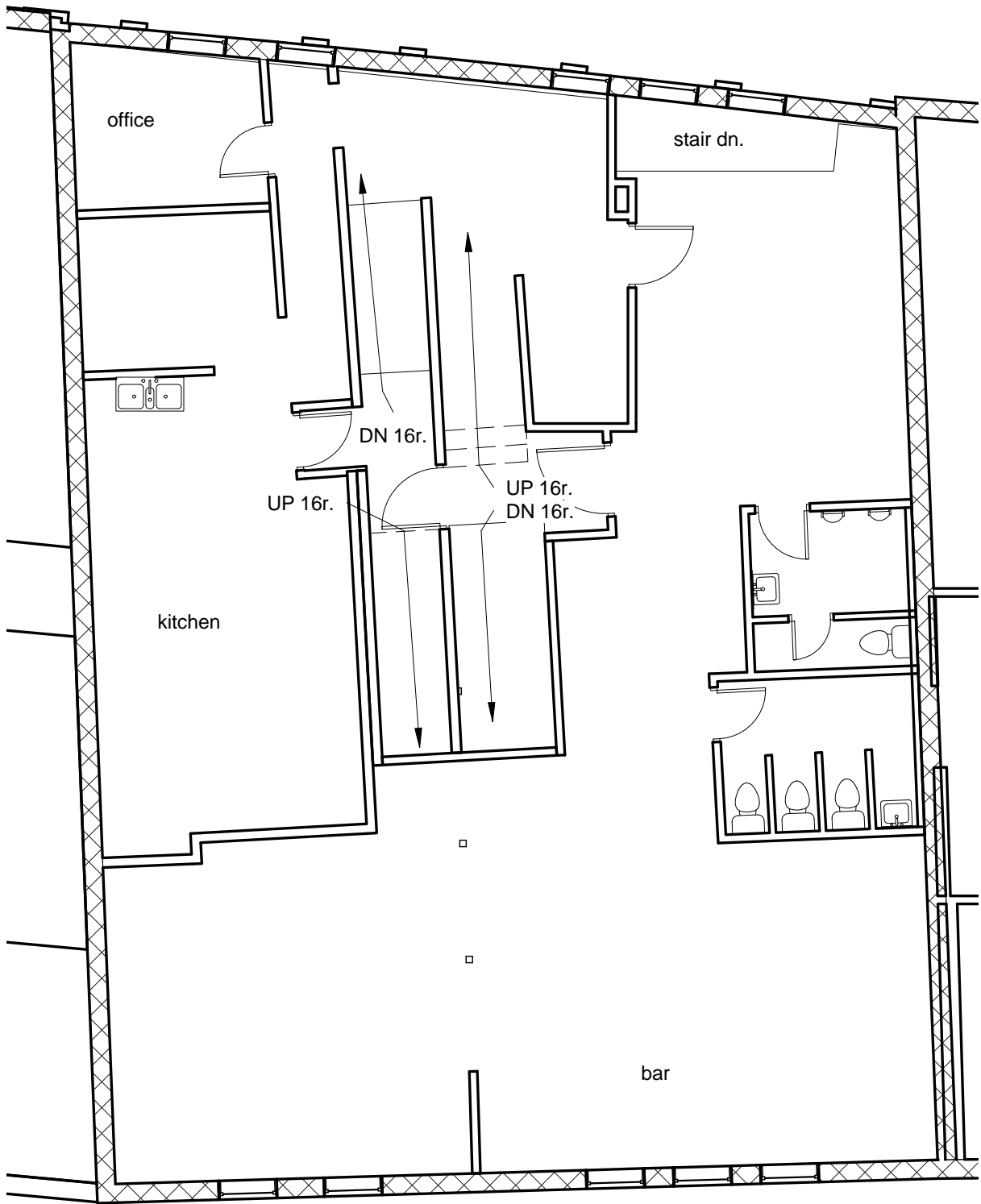
1 Level 2 @ 438 Fore 1/8" = 1'-0"
