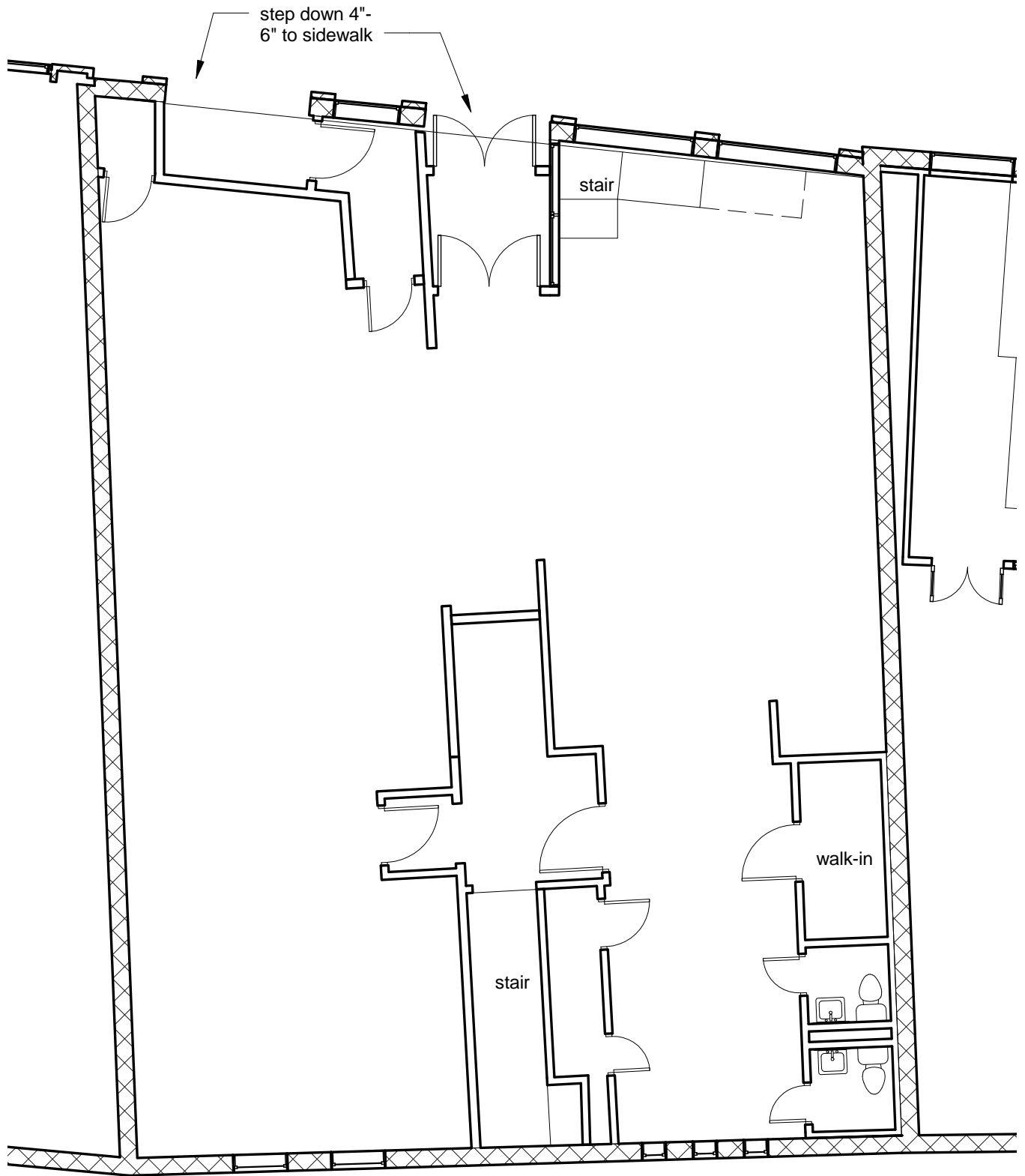
① Level 1 @ 436-438 Fore 1/8" = 1'-0"
