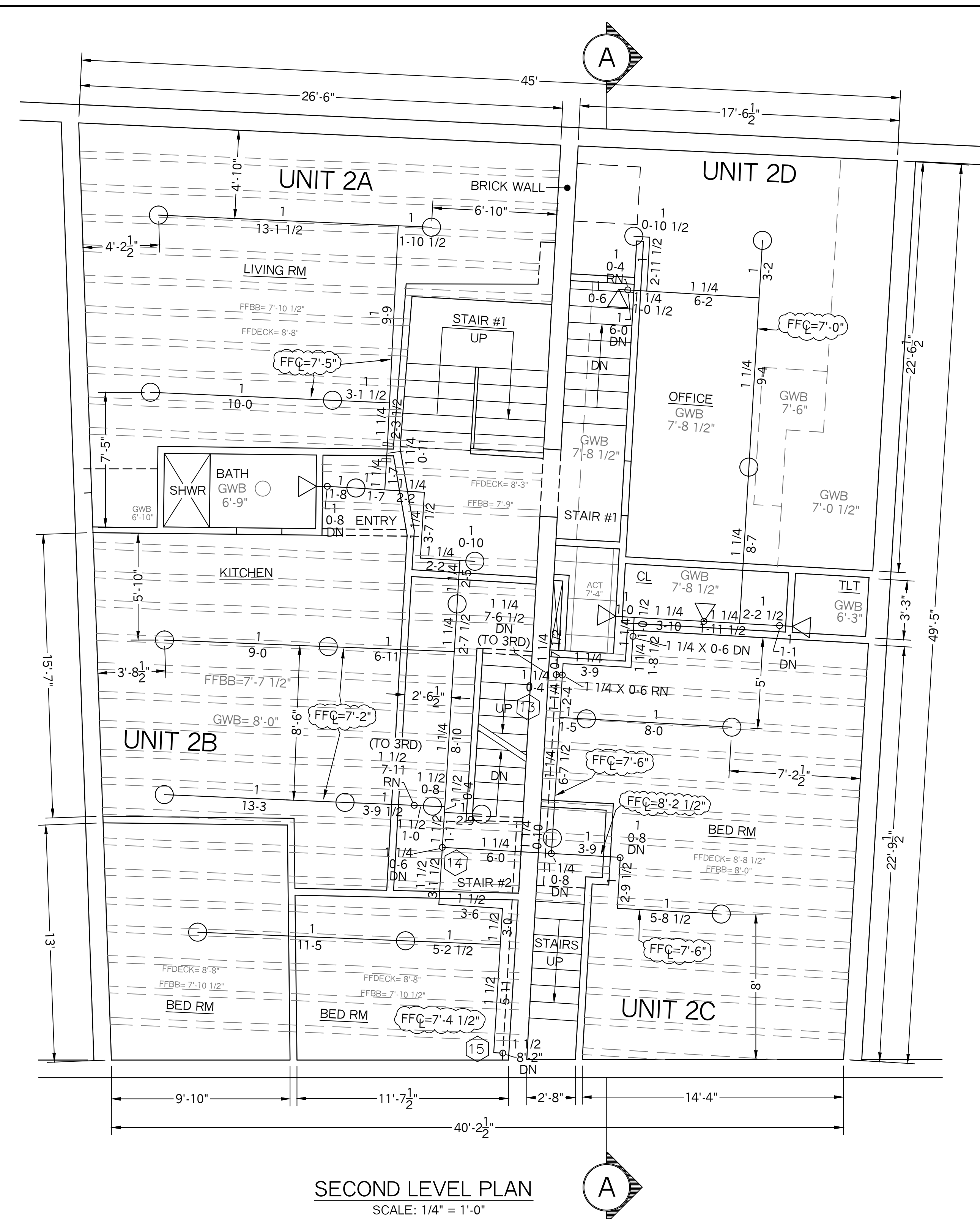
SPRINKLER HEAD INFORMATION, THIS FLOOR ONLY
