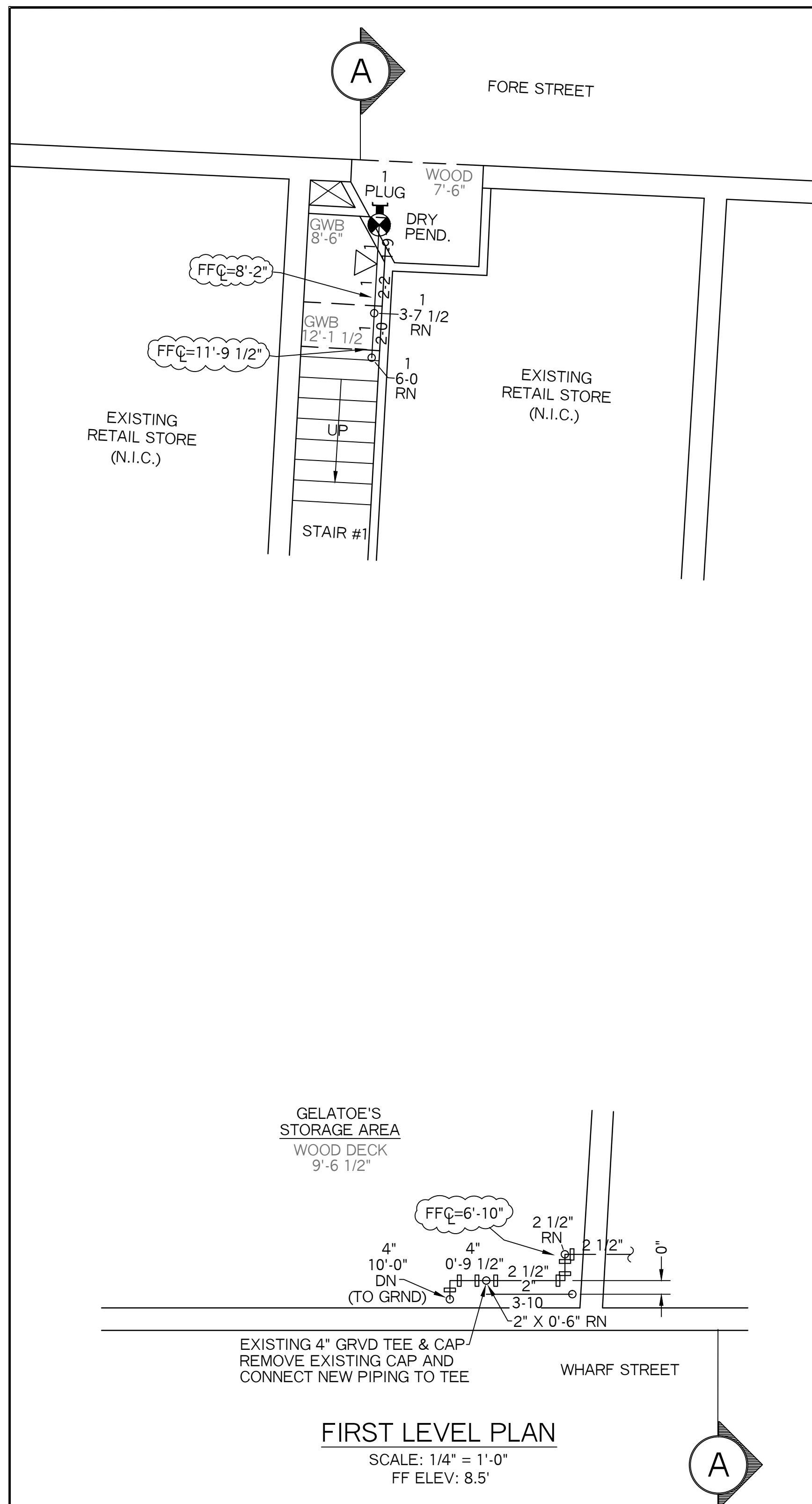
SPRINKLER HEAD INFORMATION, THIS FLOOR ONLY
