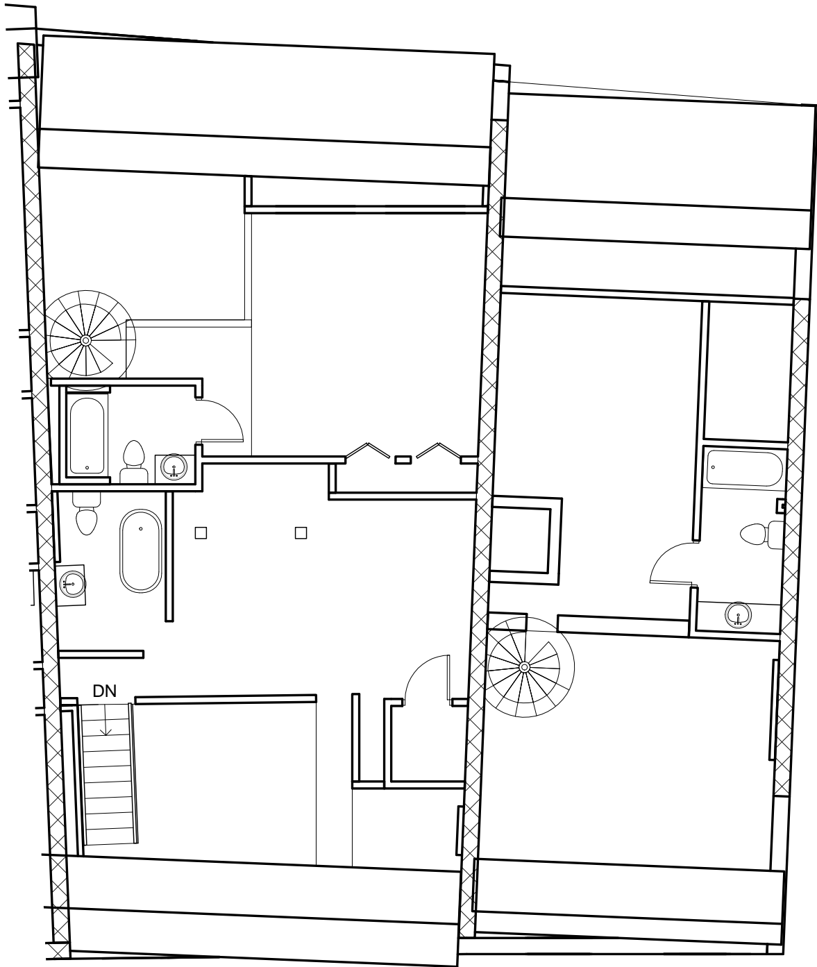
① Level 4 (loft) @ 432 Fore 1/8" = 1'-0"
