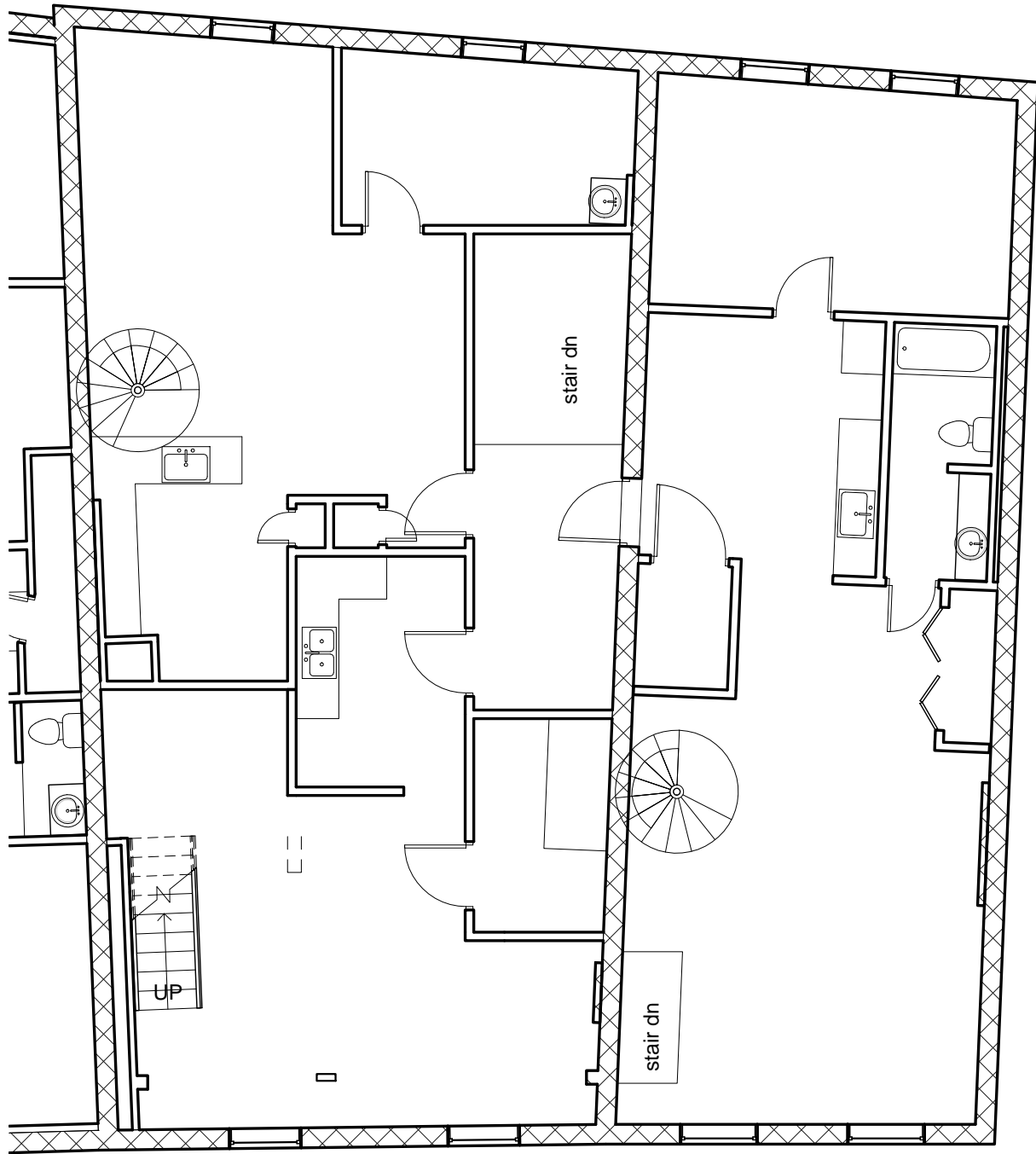
1 Level 3 @ 432-434 Fore 1/8" = 1'-0"
