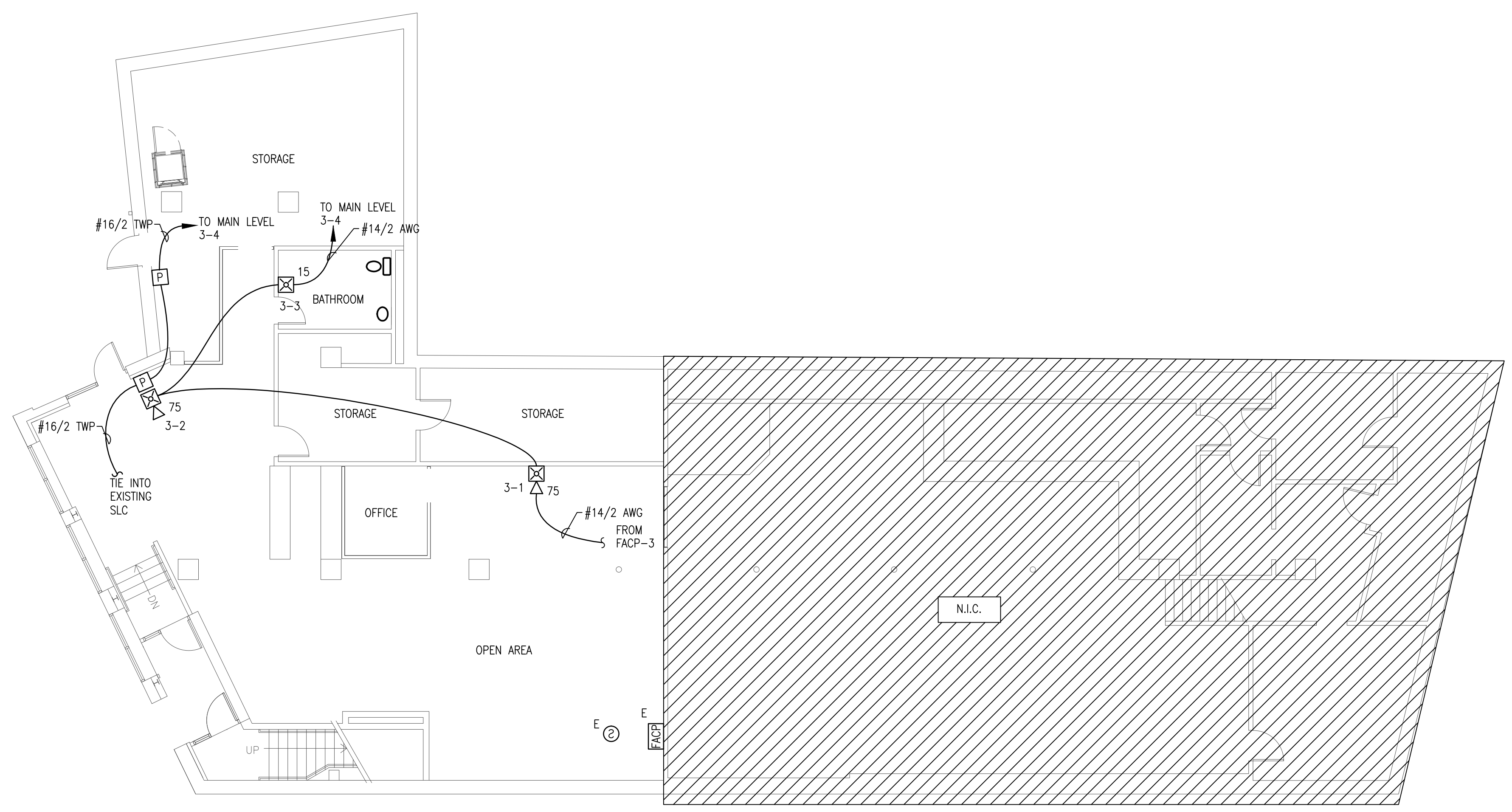
BASEMENT LEVEL FIRE ALARM PLAN SCALE: 1/8"=1'-0"
