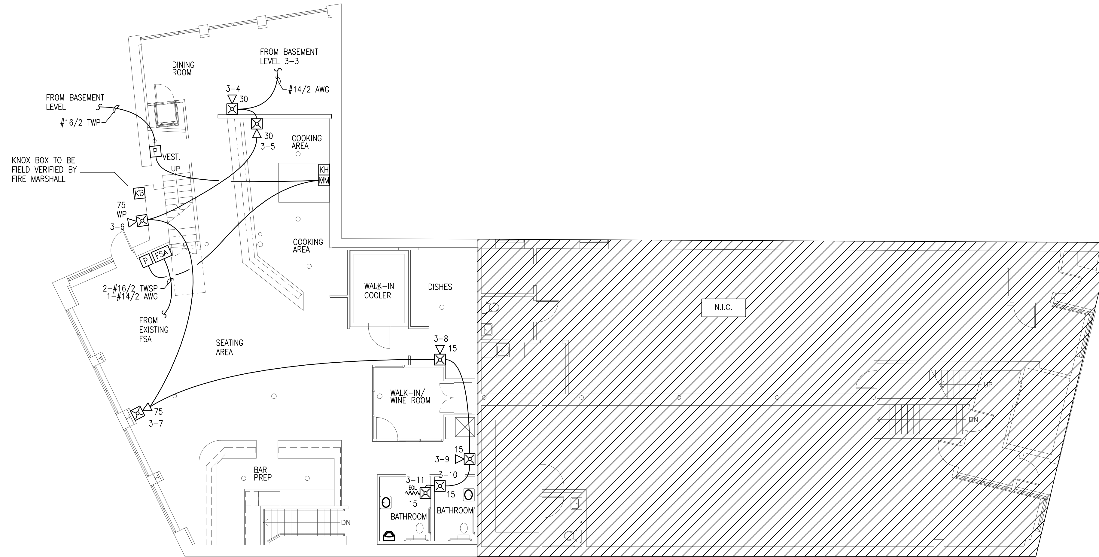
MAIN LEVEL FIRE ALARM PLAN SCALE: 1/8"=1'-0"
