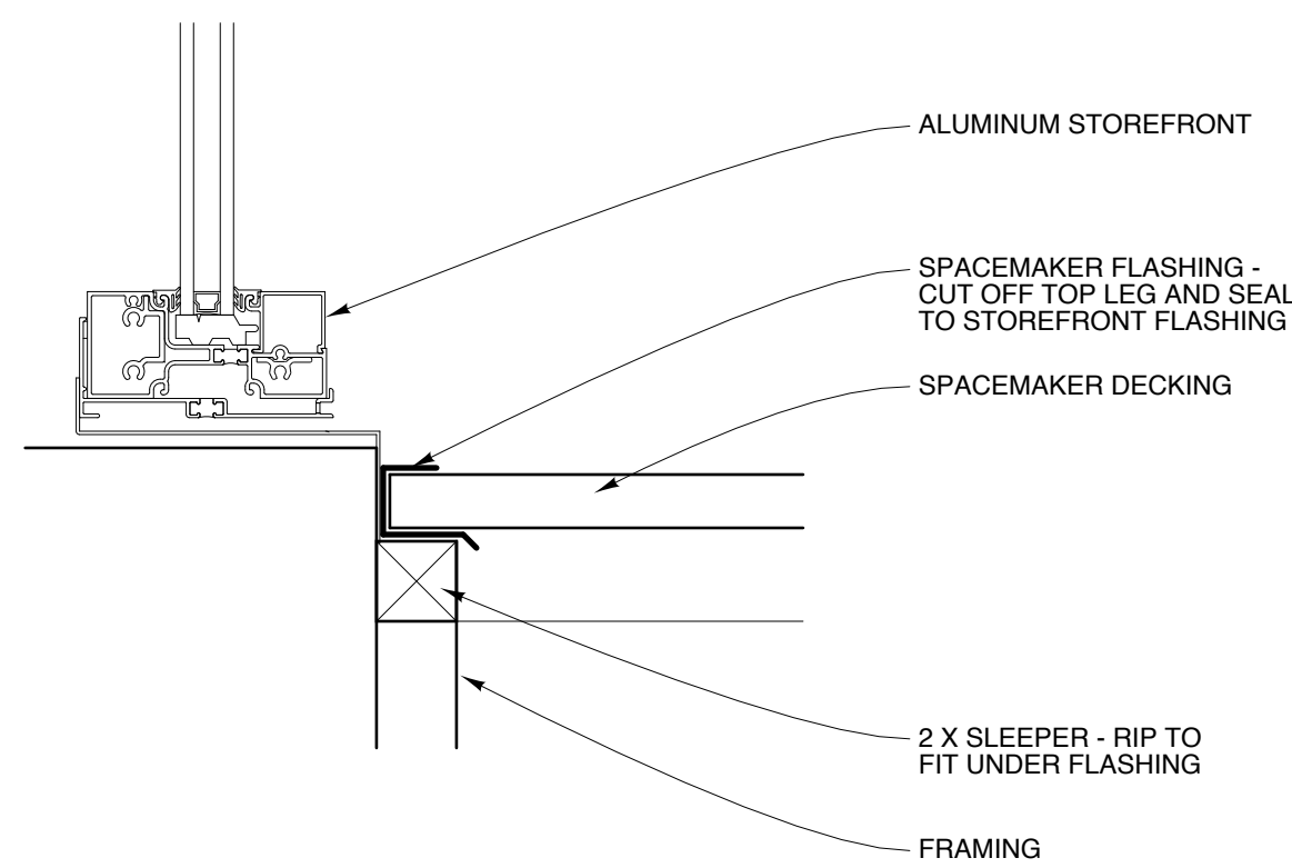
5 DETAIL AT STOREFRONT SCALE: 3" = 1'-0" 1' 2' 4' 8'
