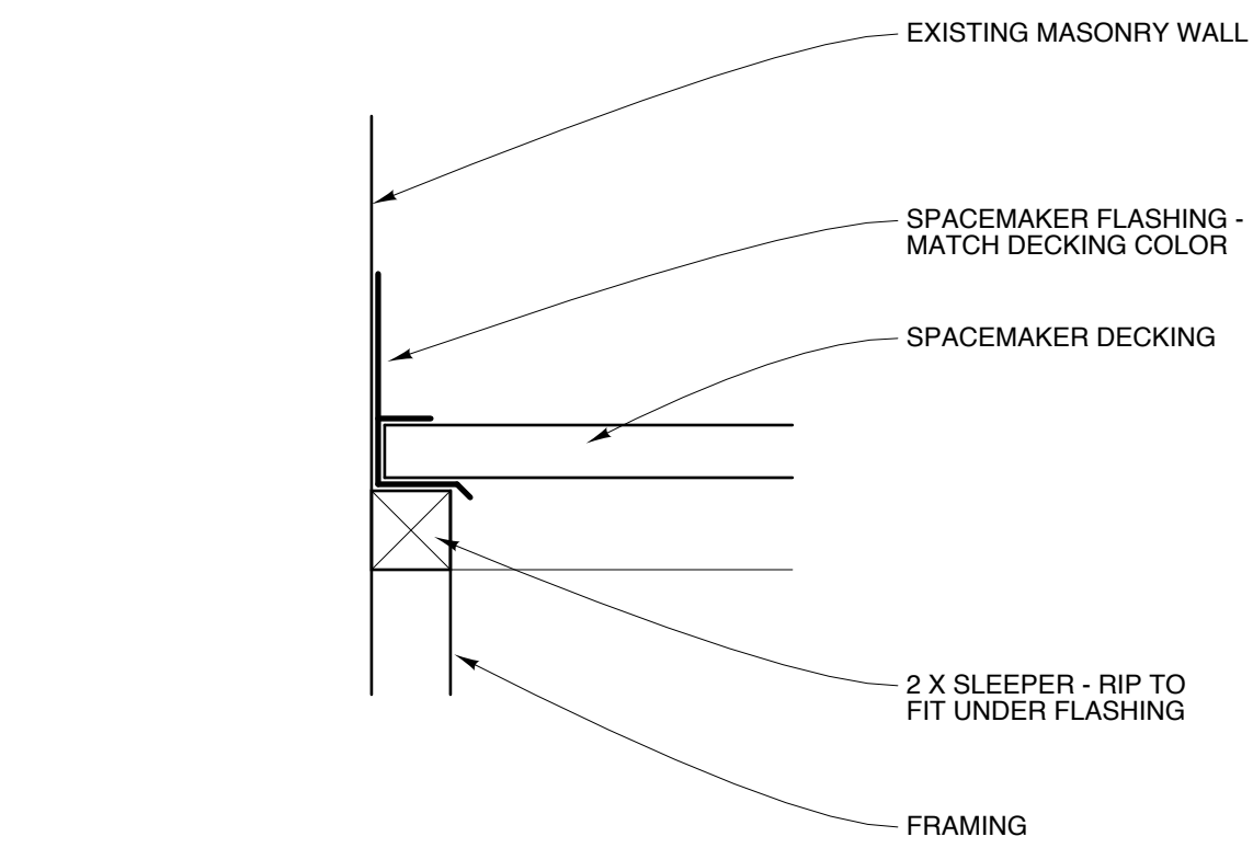
4 DETAIL AT WALL SCALE: 3" = 1'-0" 1' 2' 4' 8'
