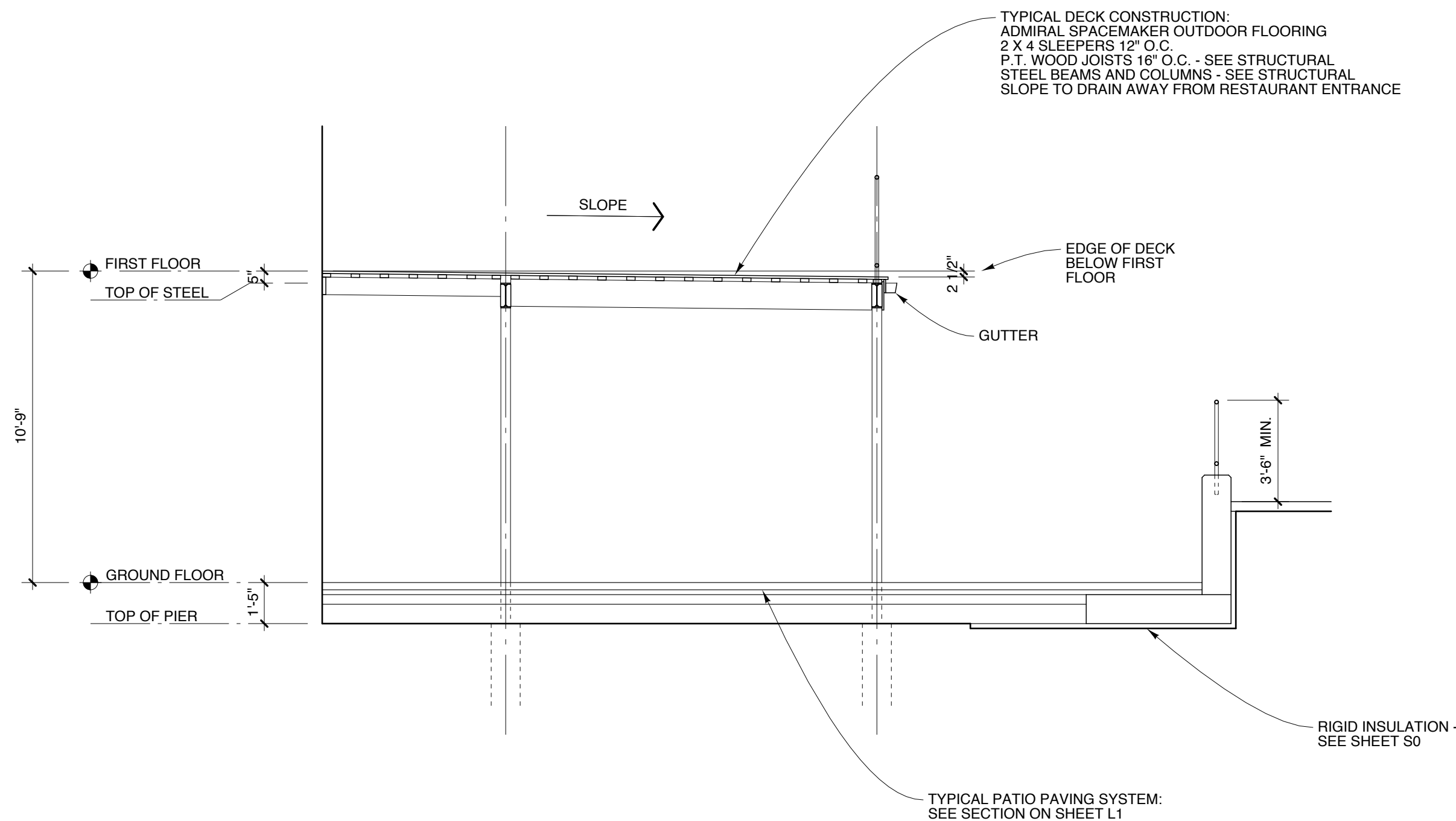
2 SECTION SCALE: 1/4" = 1'-0" 1' 2' 4' 8'
