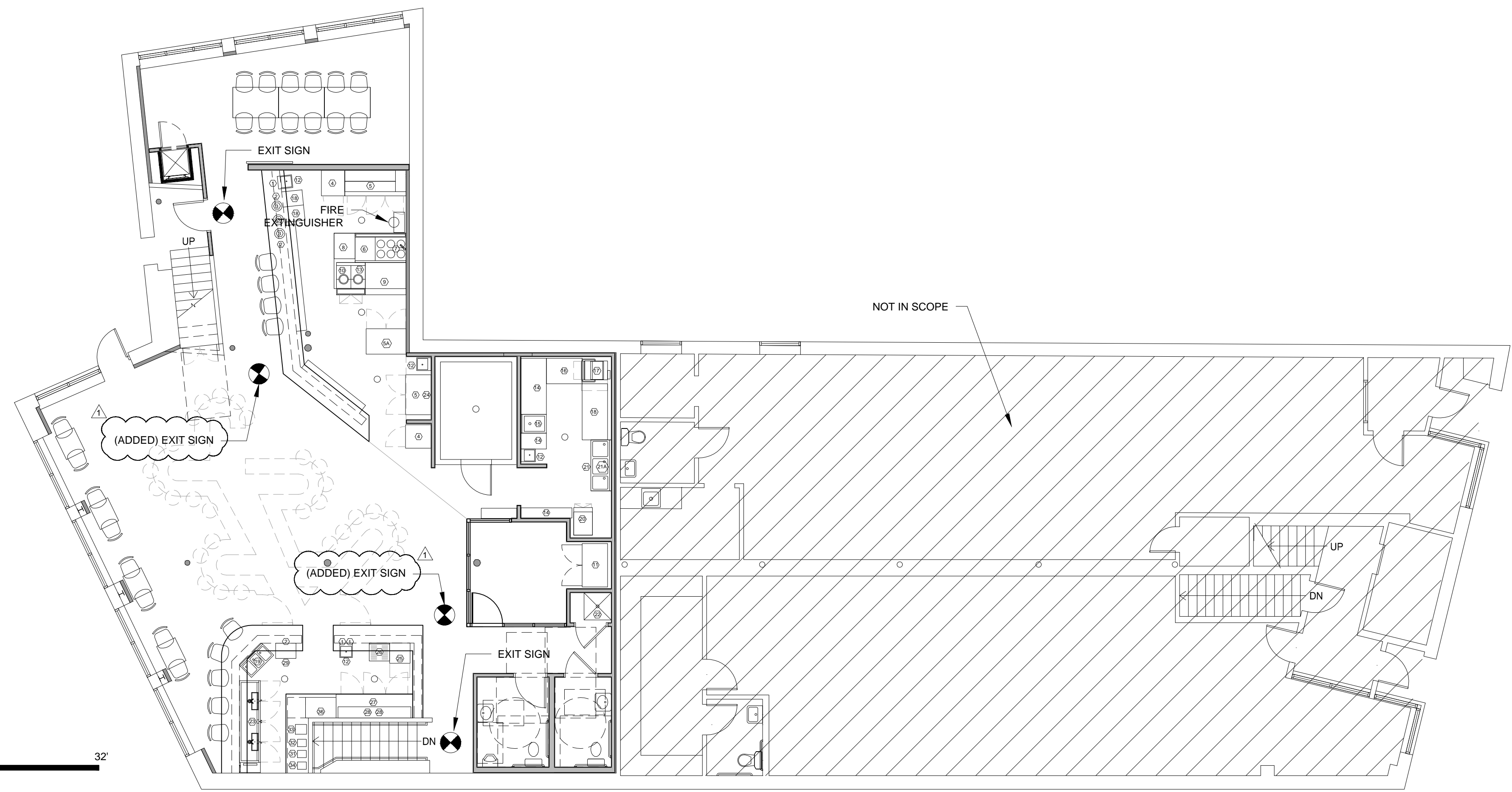
2 SECOND FLOOR CODE REVIEW PLAN 1/8" = 1'-0"
