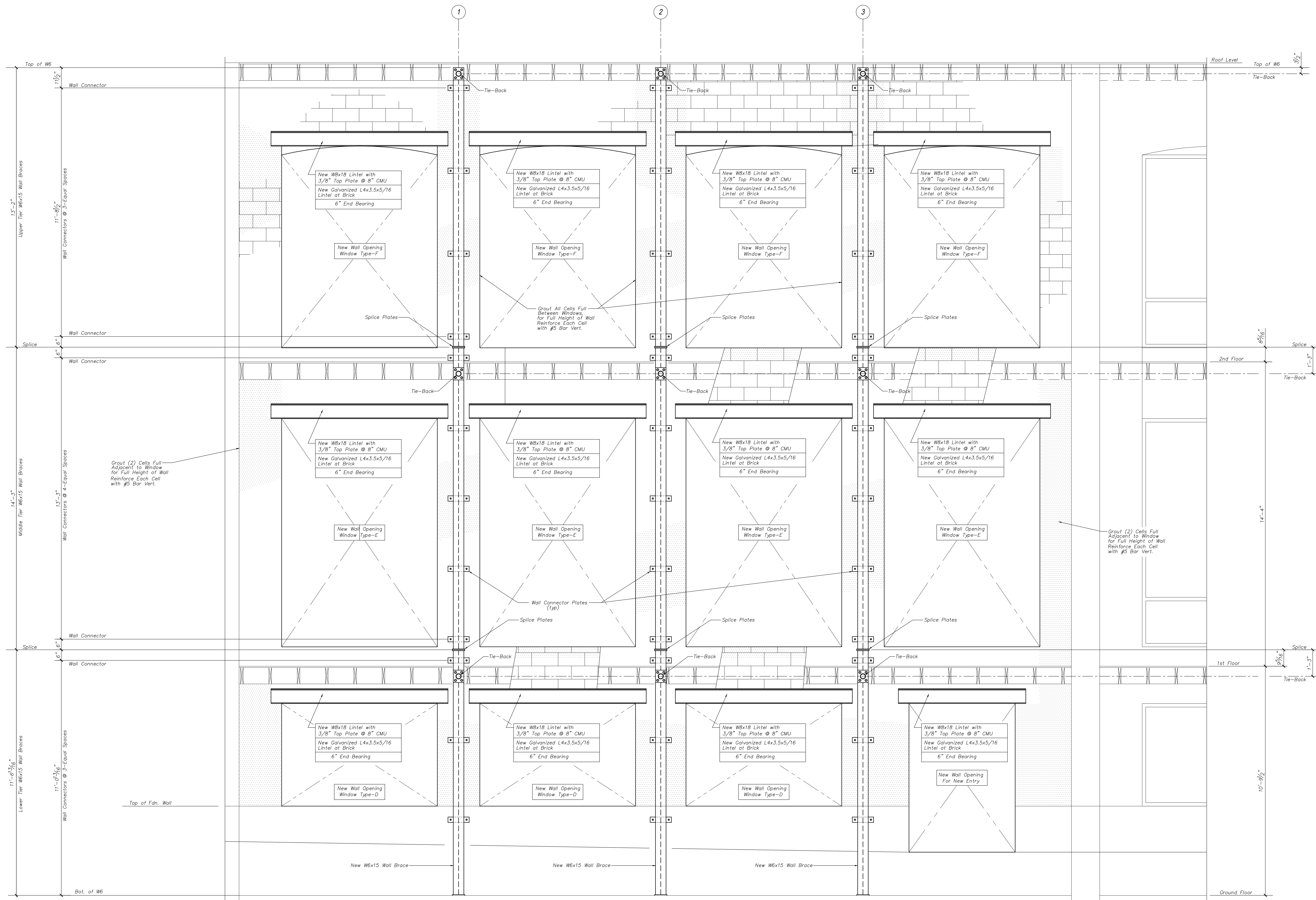
WALL FRAMING ELEVATION - SPRING STREET Scale: 1/2" = 1'-0"
