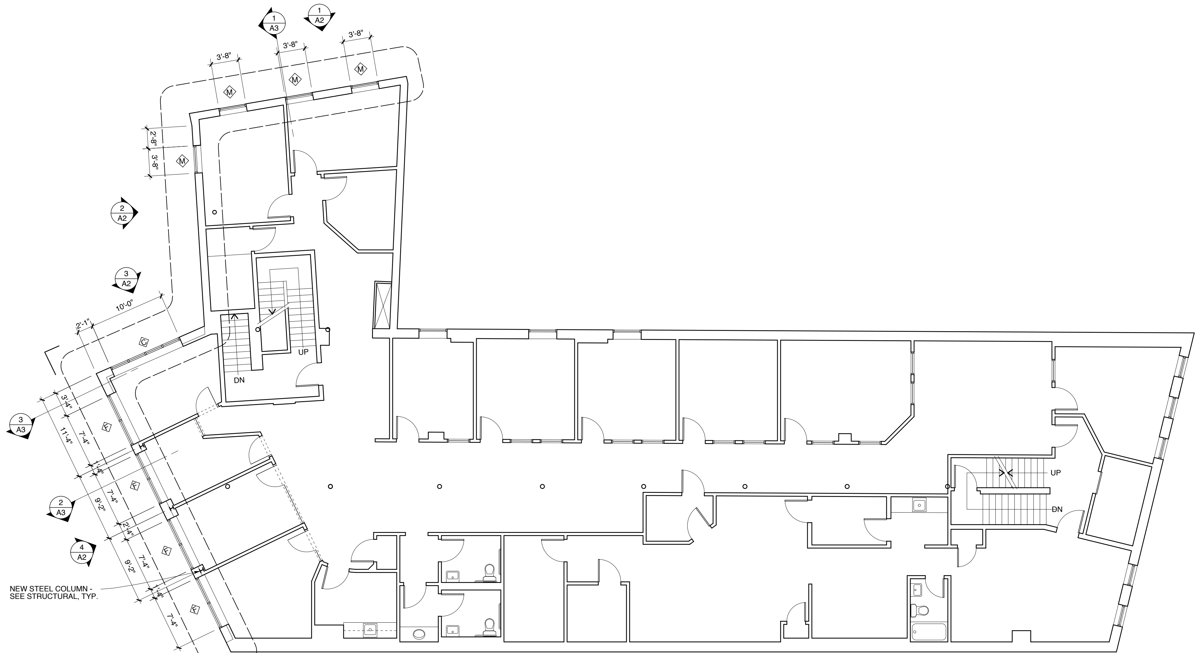
1 SECOND FLOOR PLAN SCALE: 1/8" = 1'-0" 2' 4' 8' 16'
