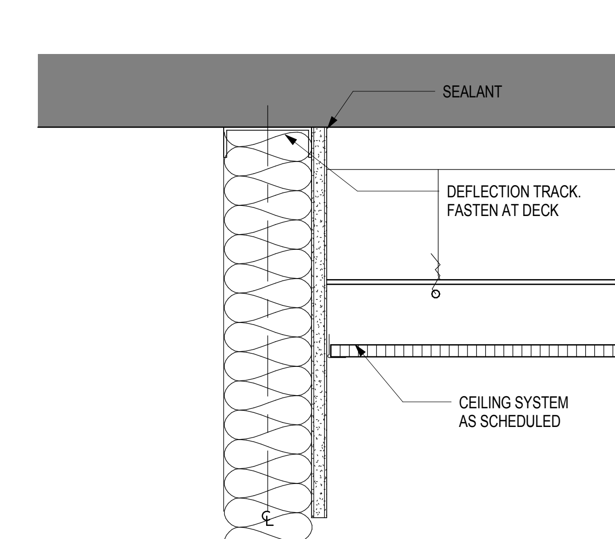
11 HEAD DETAIL - 'HD-02' SCALE: 3" = 1'-0"
