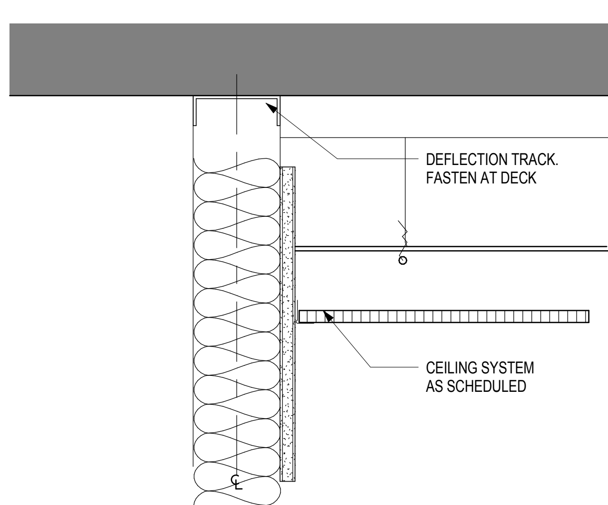
10 HEAD DETAIL - 'HD-01' SCALE: 3" = 1'-0"
