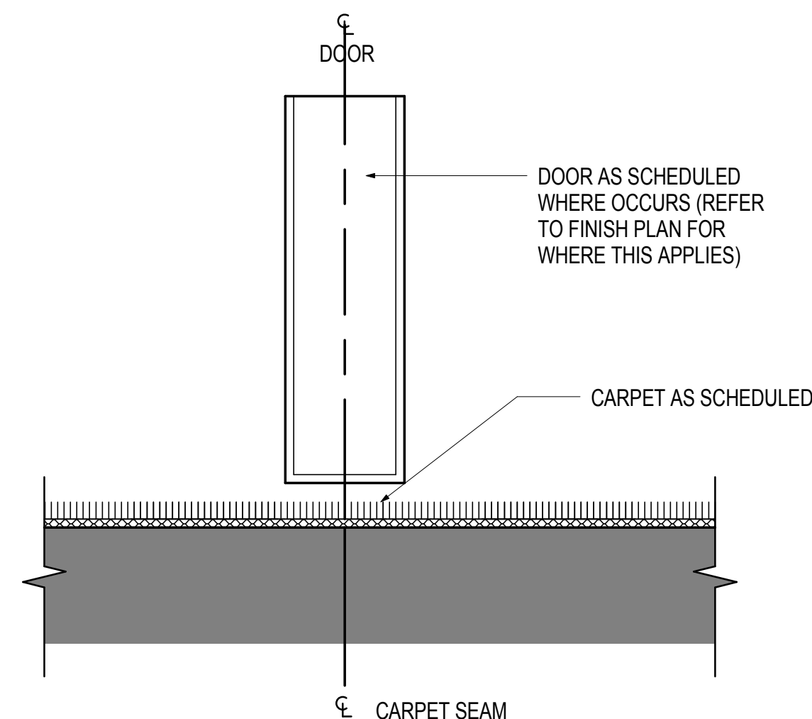
15 CARPET TO CARPET DETAIL SCALE: 6" = 1'-0"
