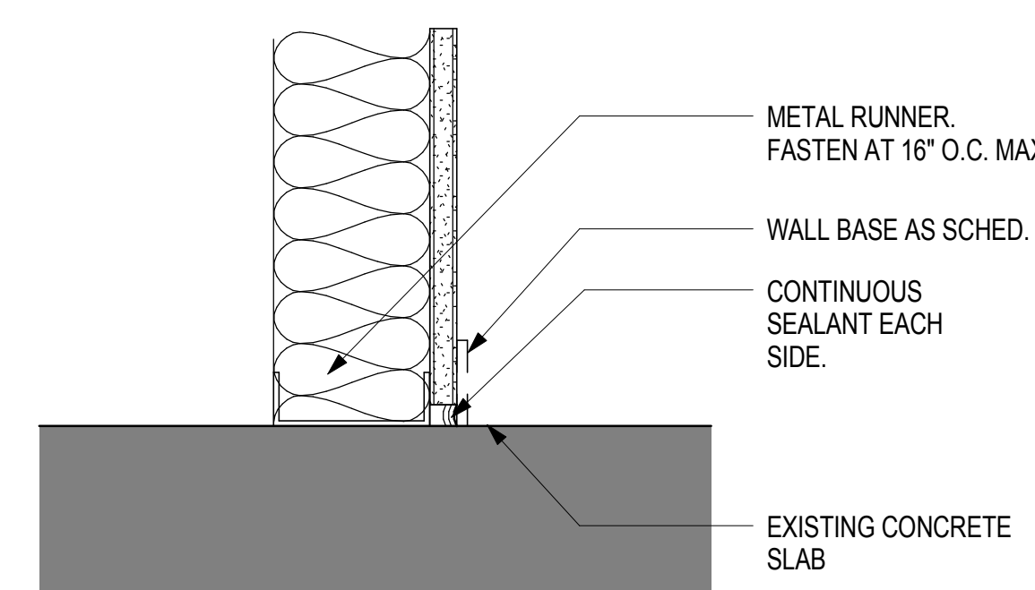
14 BASE DETAIL - 'BD-01' SCALE: 3" = 1'-0"
