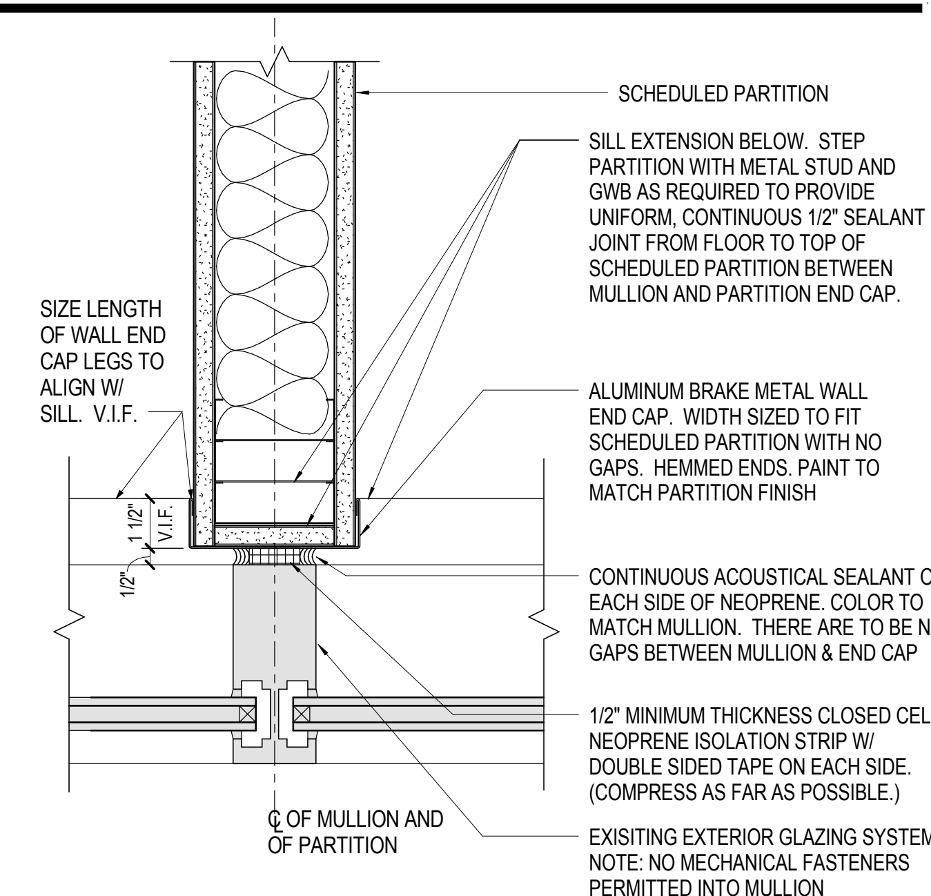
18 WALL AT MULLION SCALE: 3" = 1'-0"
