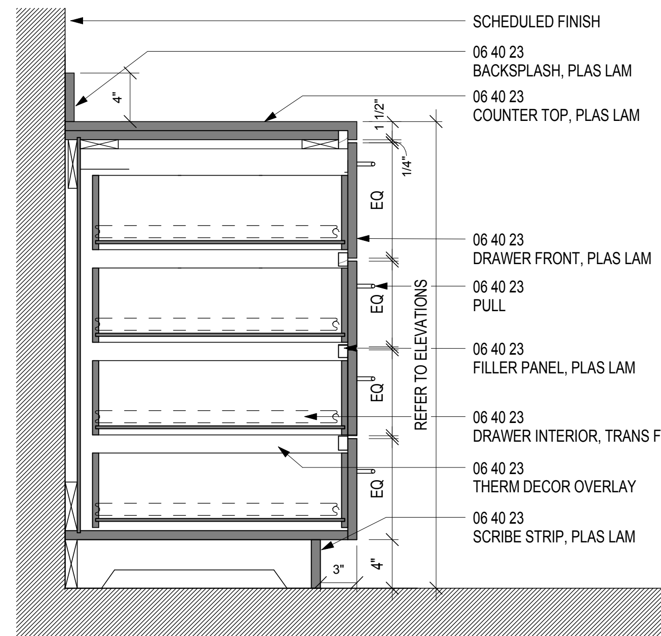
04 BASE W/ 4 DRAWERS SCALE: 1 1/2" = 1'-0"
