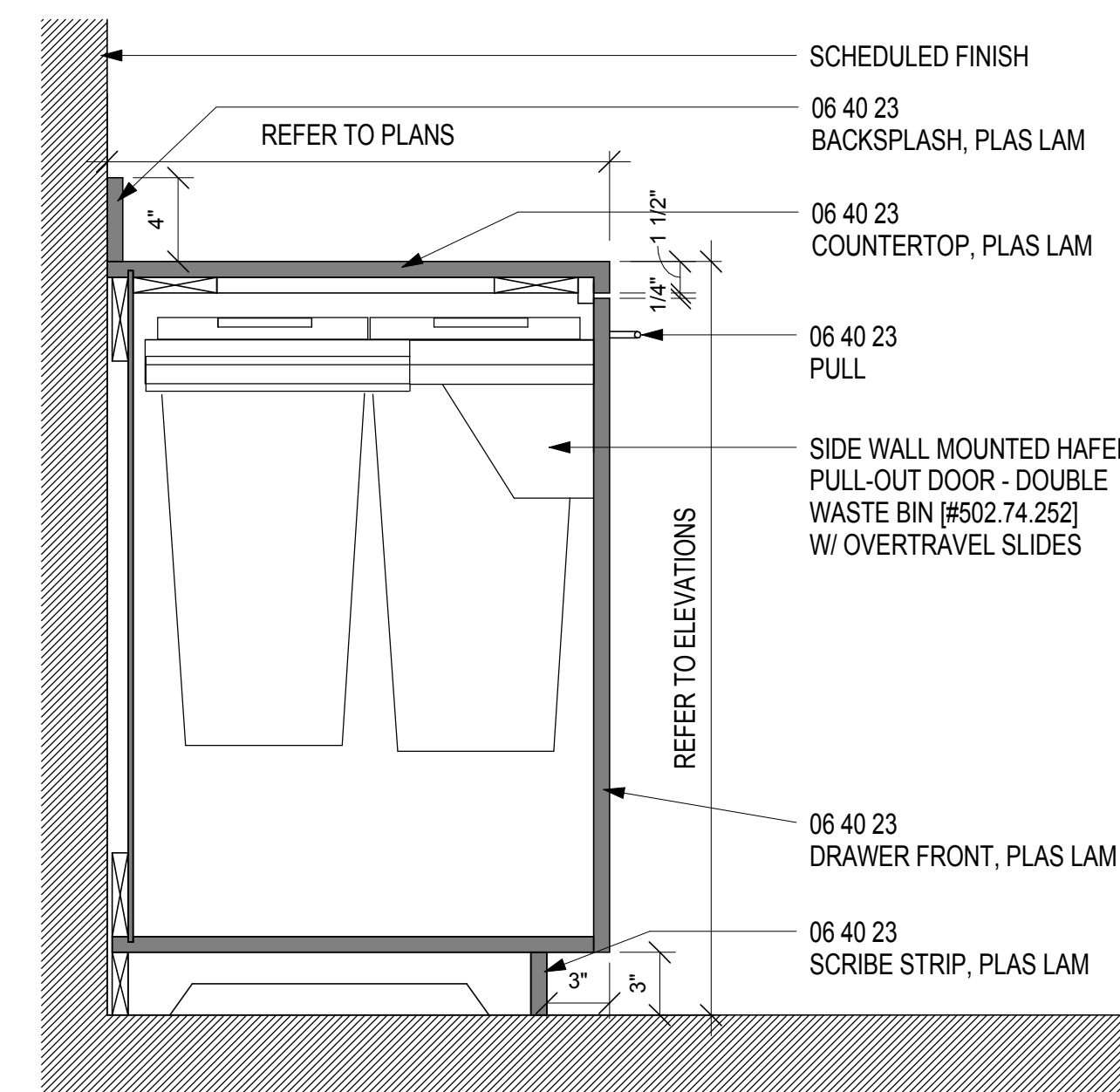
05 BASE W/ PULL-OUT TRASH SCALE: 1 1/2" = 1'-0"
