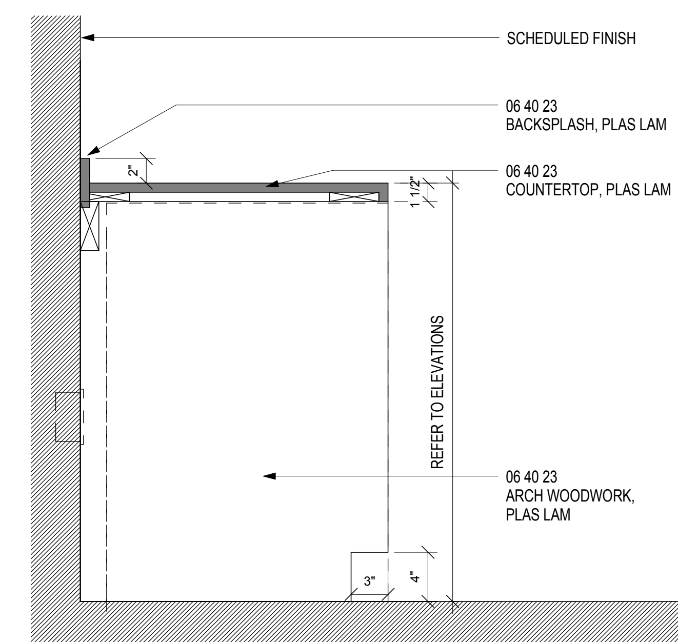
02 BASE W/ EQUIPMENT SCALE: 1 1/2" = 1'-0"
