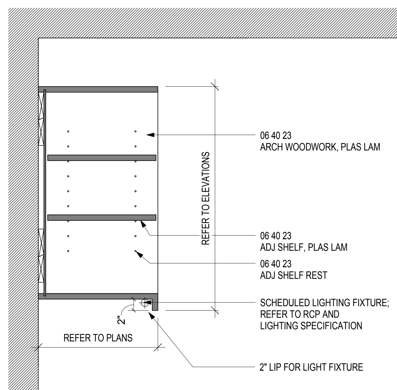
06 CABINET W/ OPEN SHELVES & UNDER LIGHT SCALE: 1 1/2" = 1'-0"
