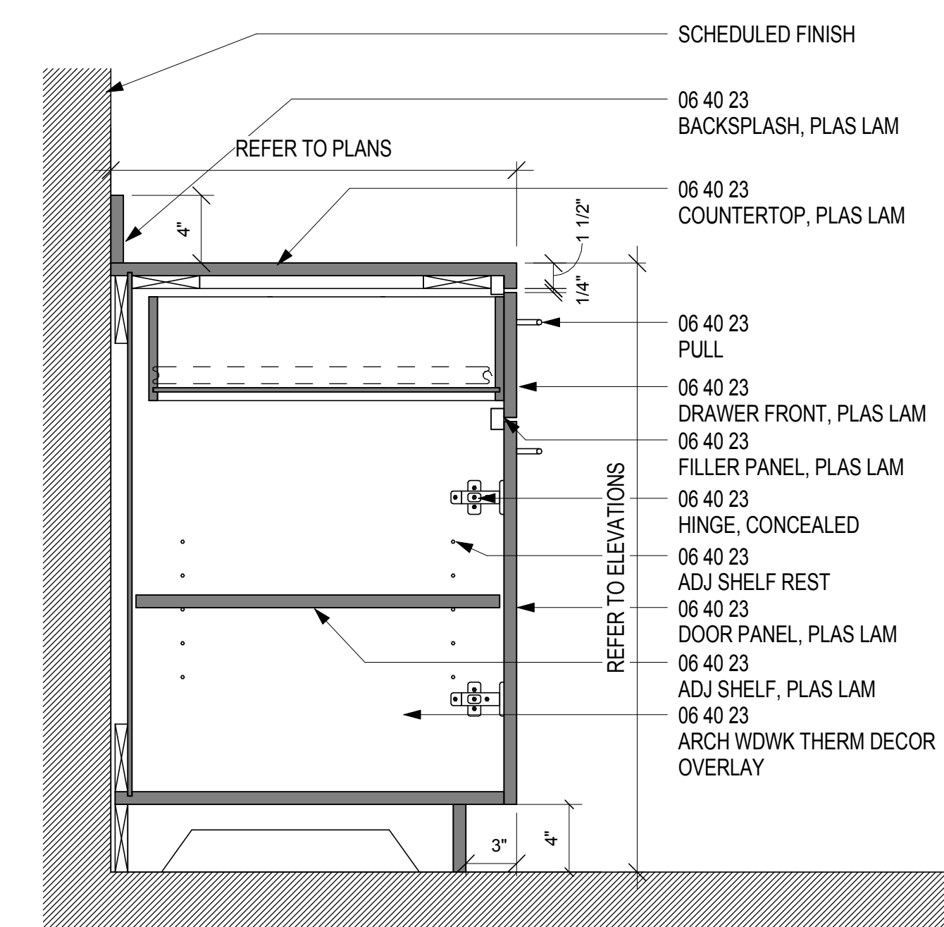
03 BASE W/ ONE DRAWER & DOOR SCALE: 1 1/2" = 1'-0"
