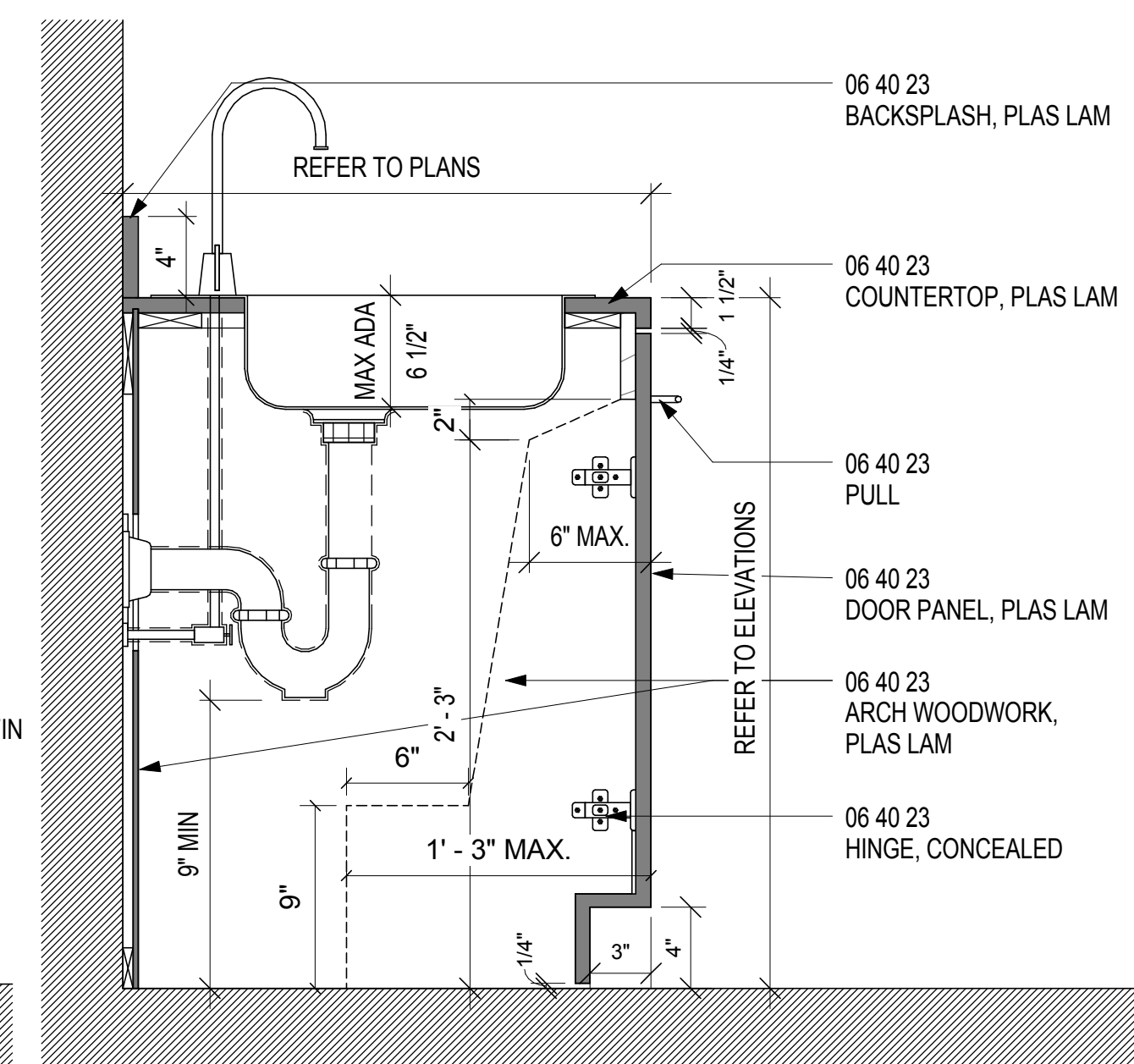
01 ADA CABINET W/ SINK SCALE: 1 1/2" = 1'-0"
