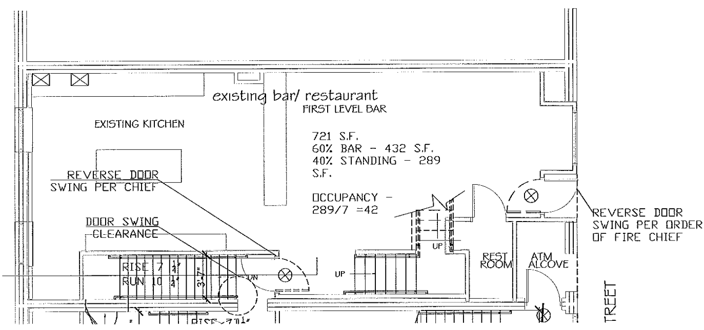
1 SLICE BAR FIRST FLOOR A1.01 1/4" = 1'-0"
