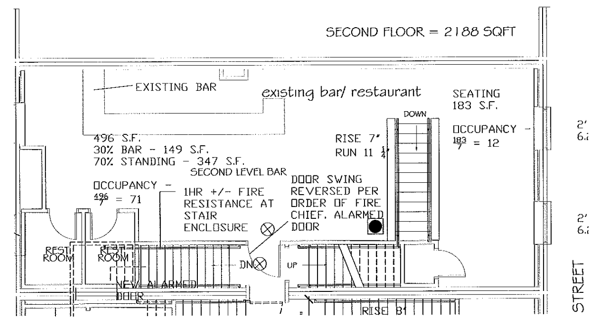
2 SLICE BAR SECOND FLOOR A1.01 1/4" = 1'-0"
