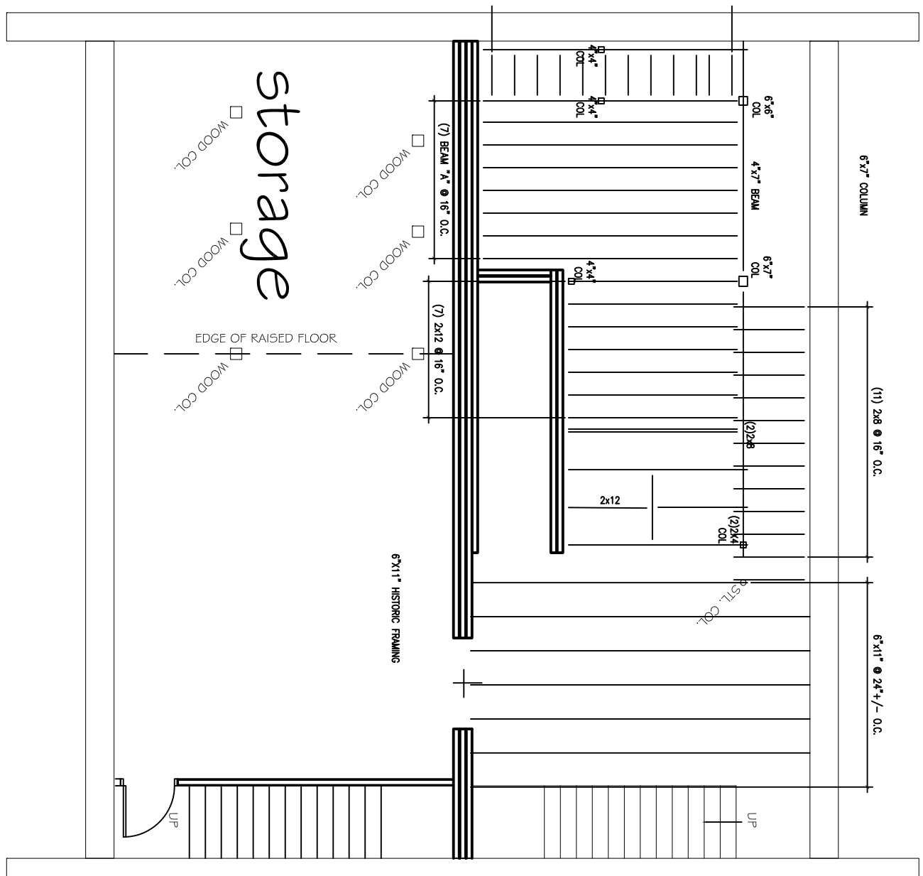
1 BASEMENT FRAMING PLAN A1.02 1/8" = 1'-0"
