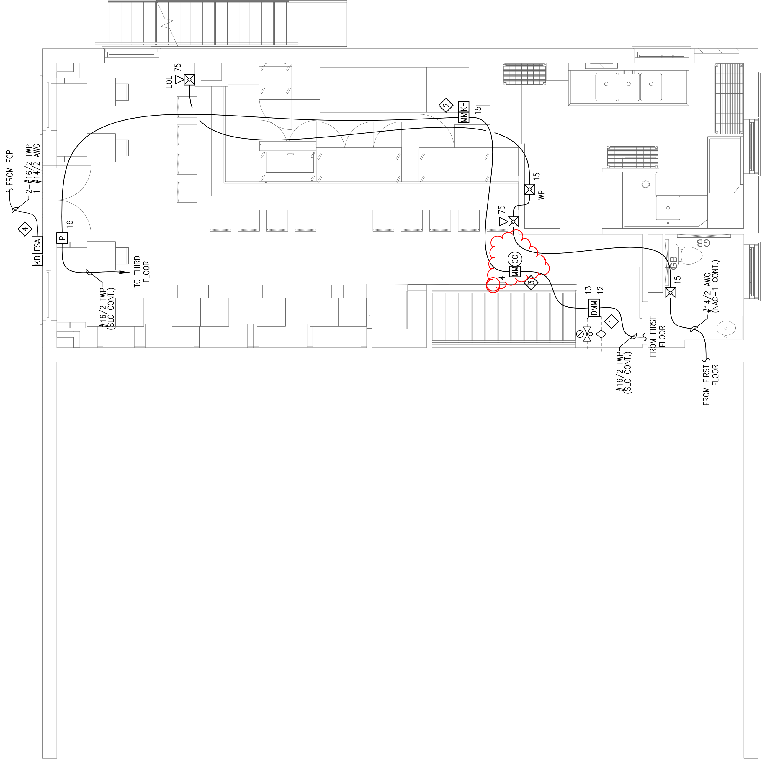
SECOND FLOOR FIRE ALARM PLAN SCALE: 1/4"=1'-0"
