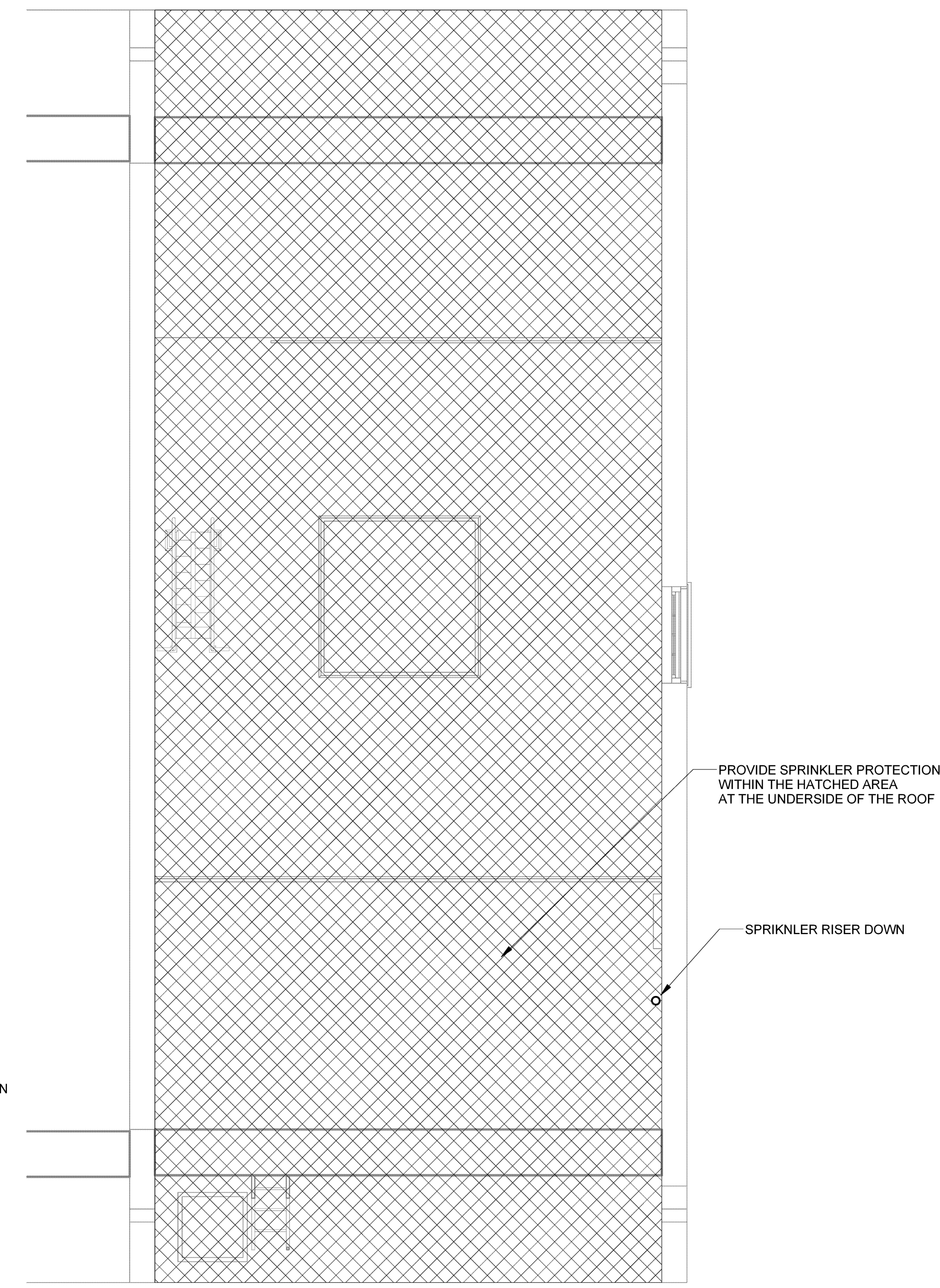
3 FIFTH FLOOR FIRE PROTECTION SCALE: 1/4" = 1'-0"
