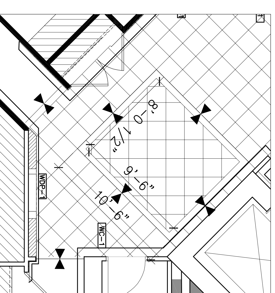
2 DETAIL OF RECEPTION SCALE: 1/4"=1'-0"
