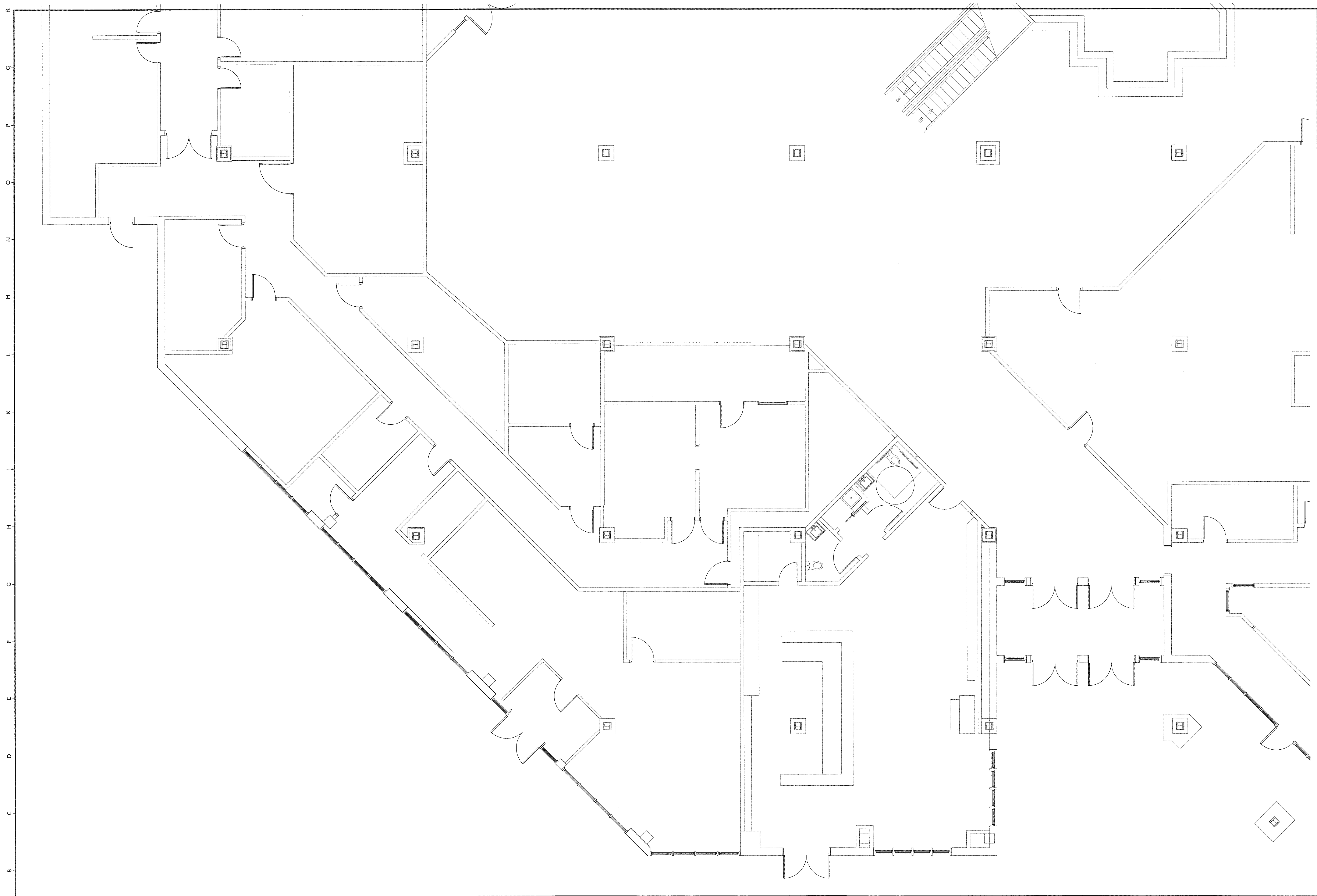
AI EXISTING CONDITIONS - FIRST FLOOR PLAN
