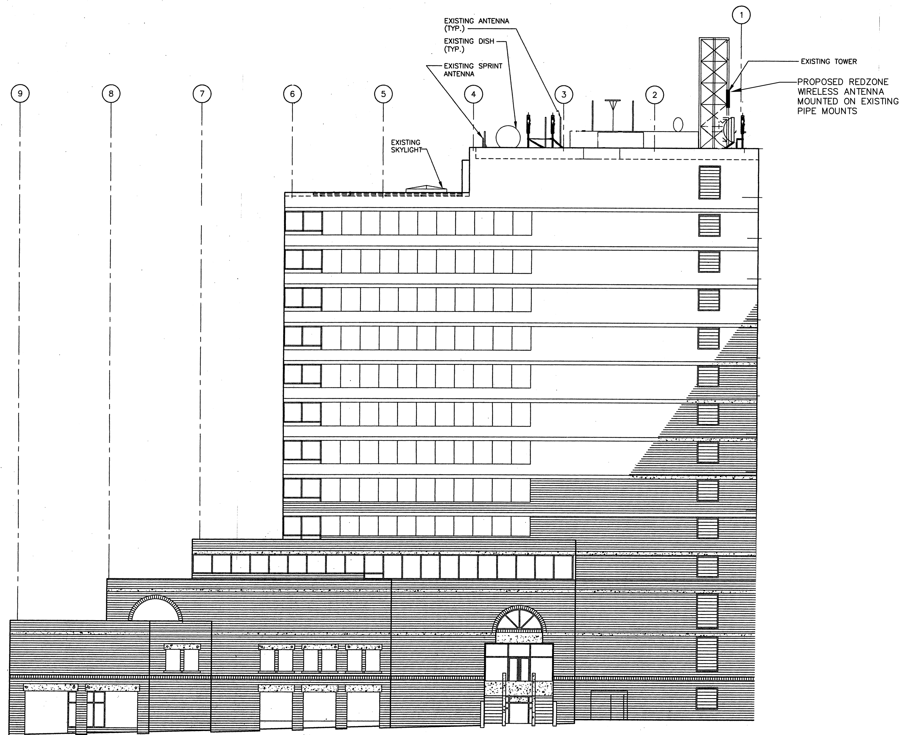
1 TEMPLE STREET (EAST) ELEVATION E-2 SCALE: 1/16"=1'
