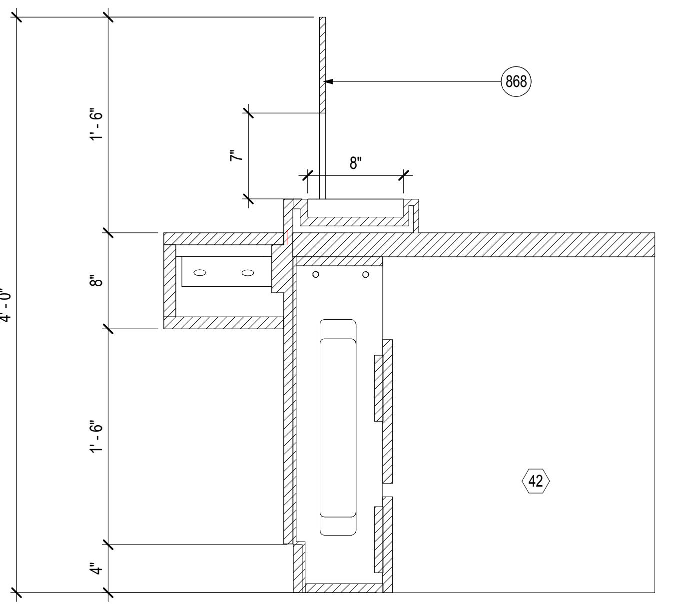
TELLER STATION ELEVATION - PUBLIC SIDE SCALE: 1/2" = 1'-0"
