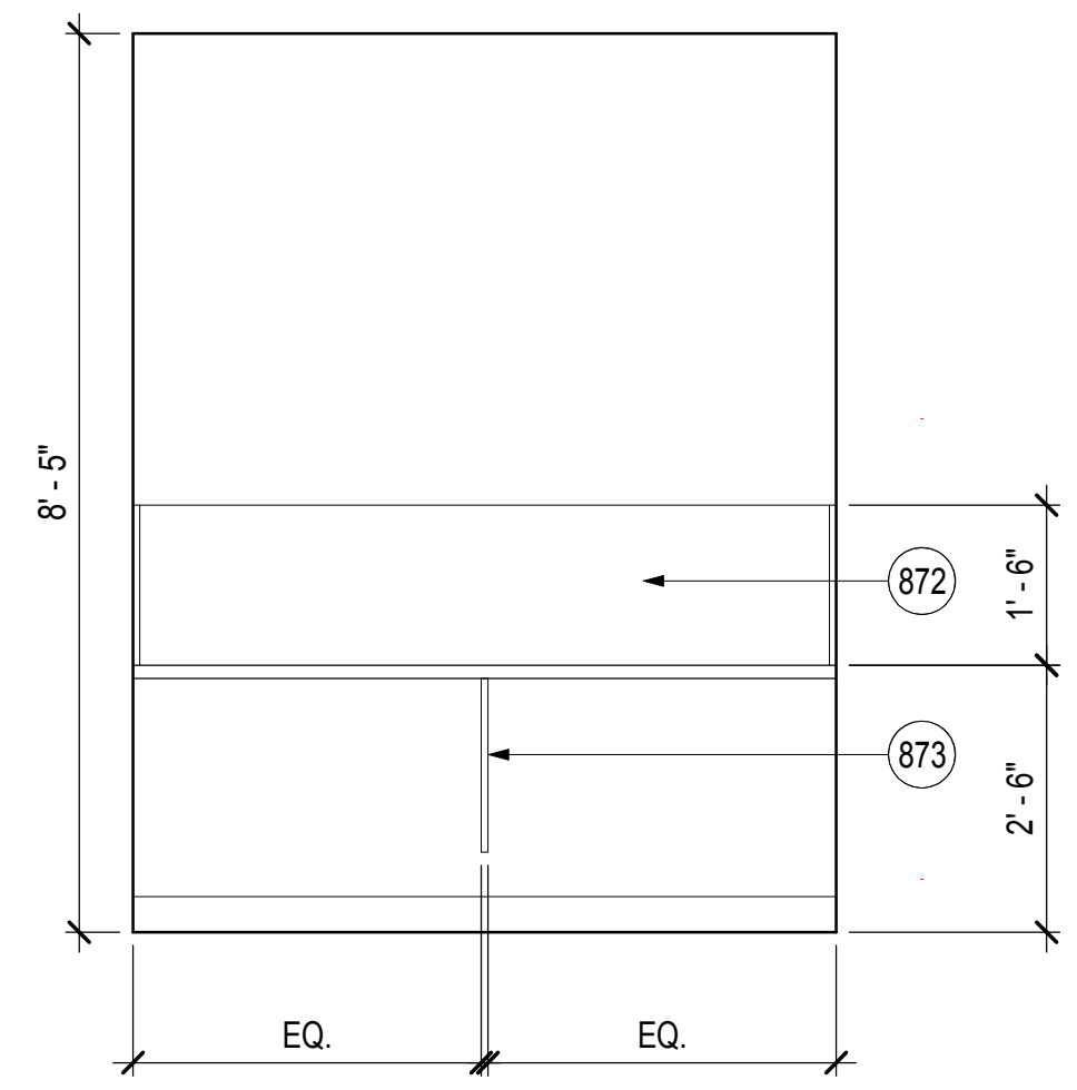
COUPON BOOTH ELEVATION SCALE: 1/2" = 1'-0"
