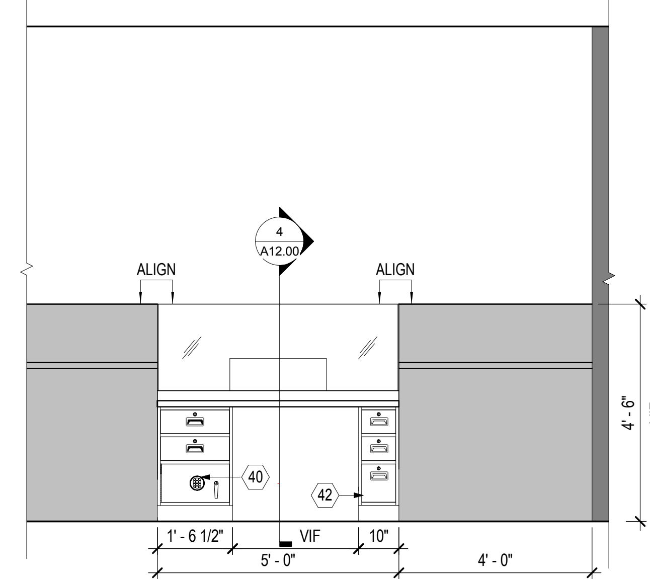
TELLER STATION ELEVATION - TELLER SIDE SCALE: 1/2" = 1'-0"
