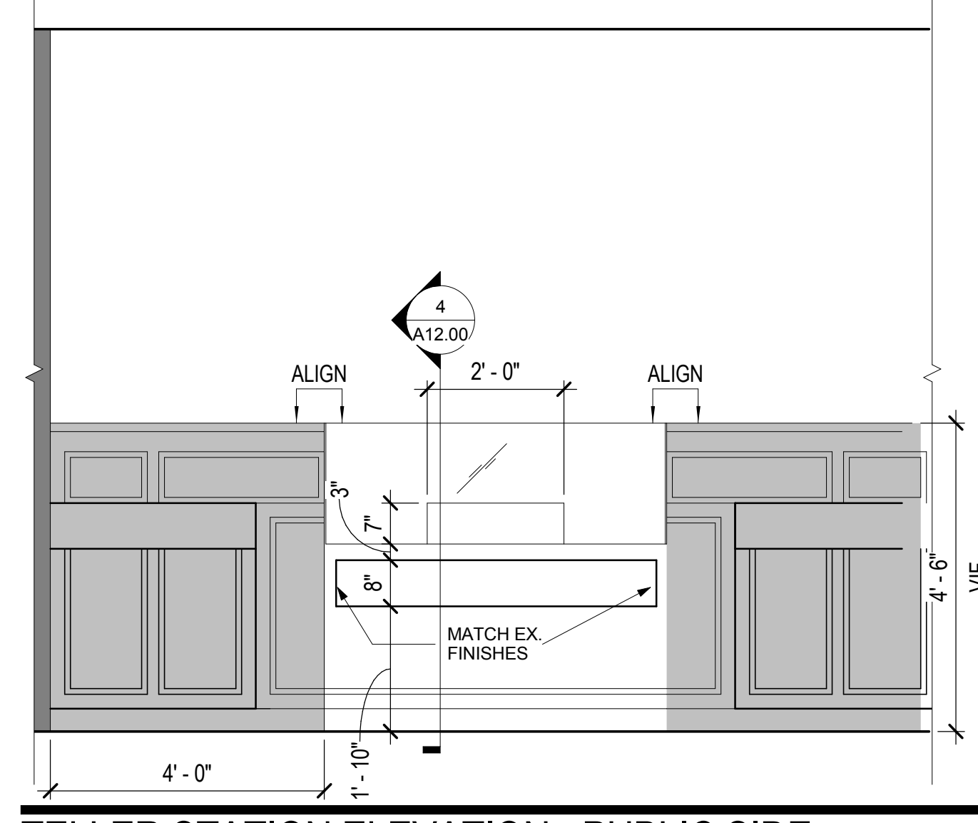
TELLER STATION ELEVATION - PUBLIC SIDE SCALE: 1/2" = 1'-0"
