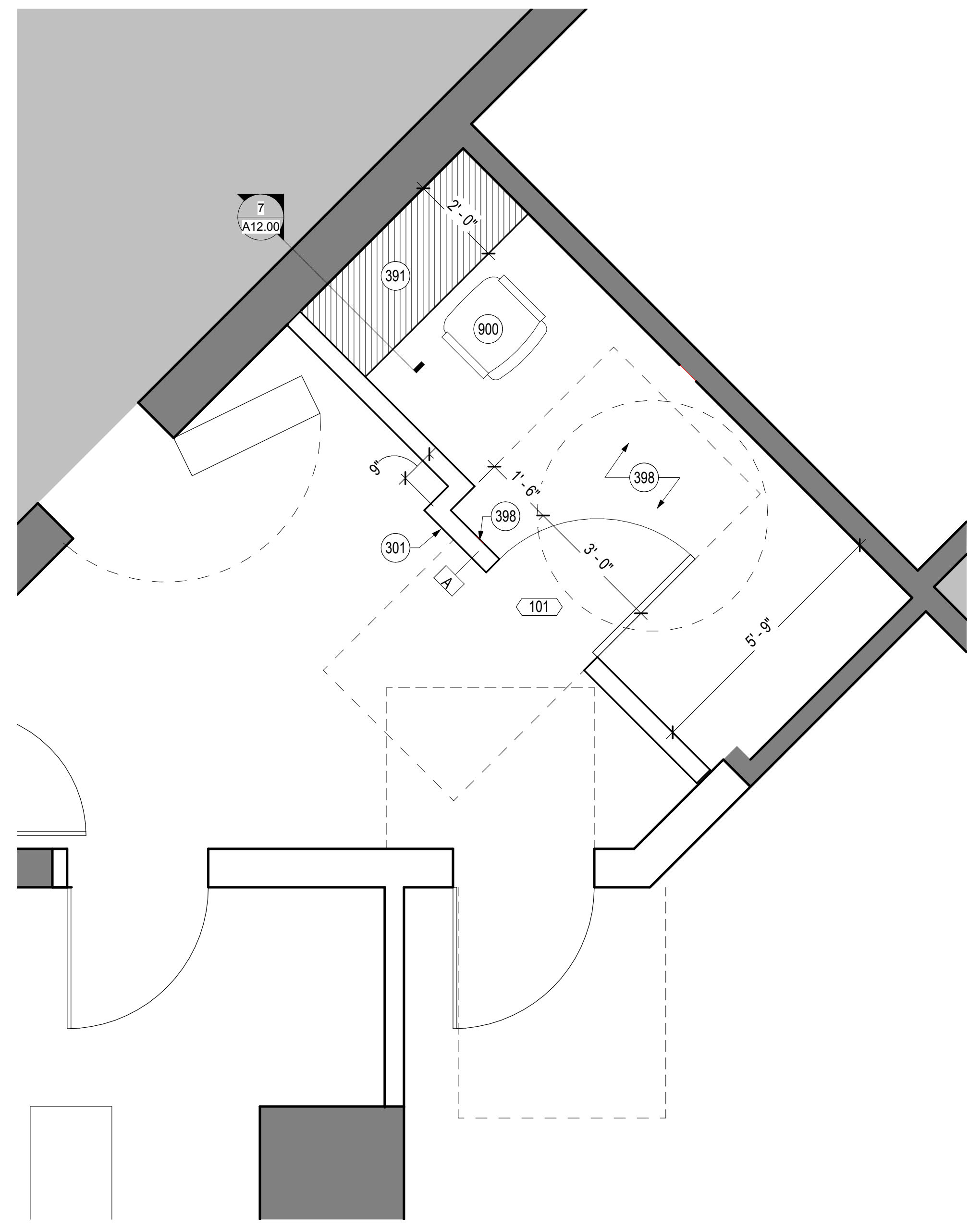
CONSTRUCTION PLAN SCALE: 1/2" = 1'-0"
