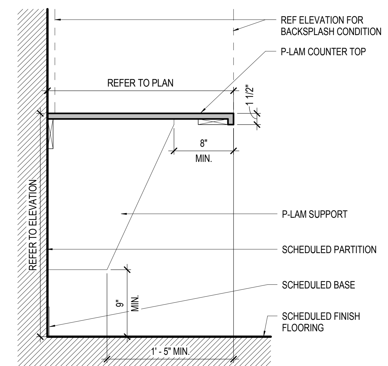
ADA COUNTER SECTION SCALE: 1 1/2" = 1'-0"
