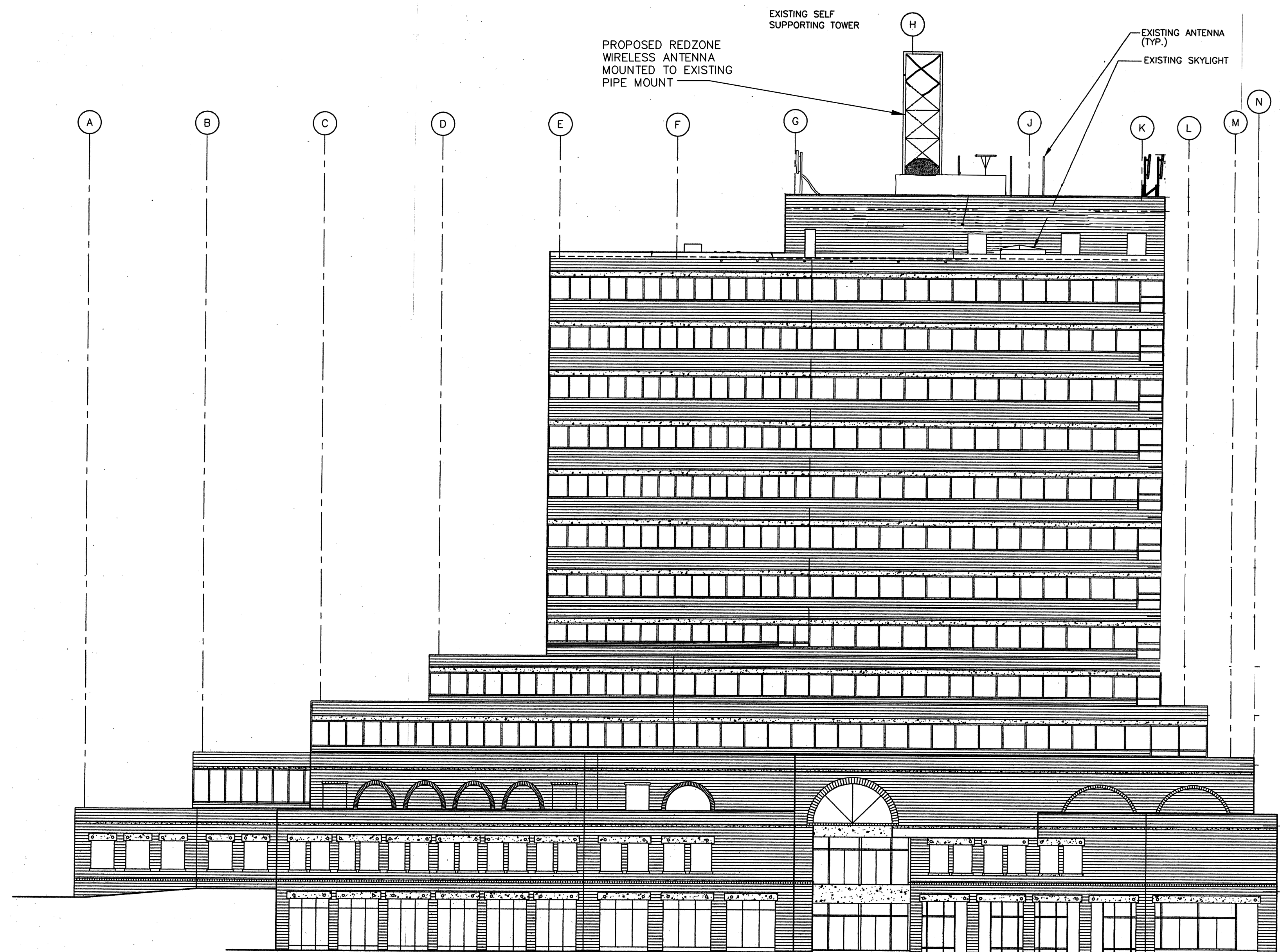
1 MIDDLE STREET (WEST) ELEVATION E-4 SCALE: 1/16"=1'
