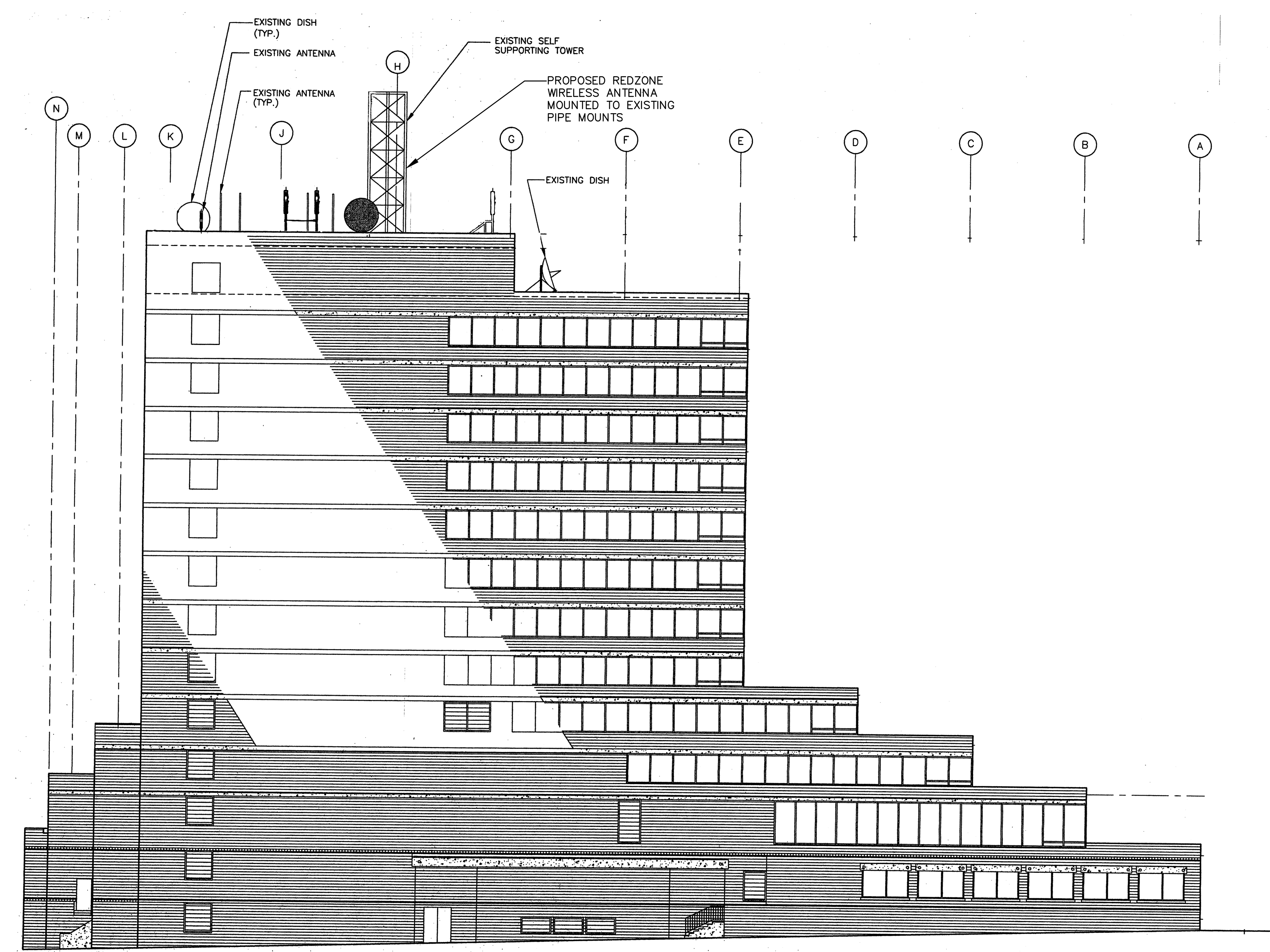
1 FEDERAL STREET (NORTH) ELEVATION E-3 SCALE: 1/16"=1'
