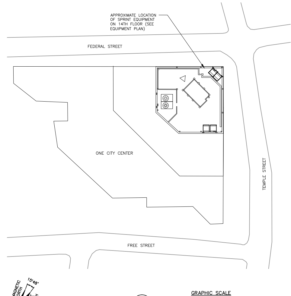
SITE PLAN SCALE: 1/32"=1'-0"
