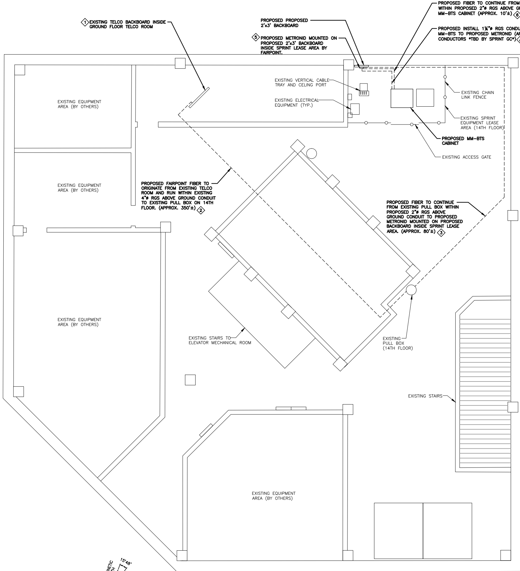
EQUIPMENT PLAN SCALE: 1/4"=1'-0"
