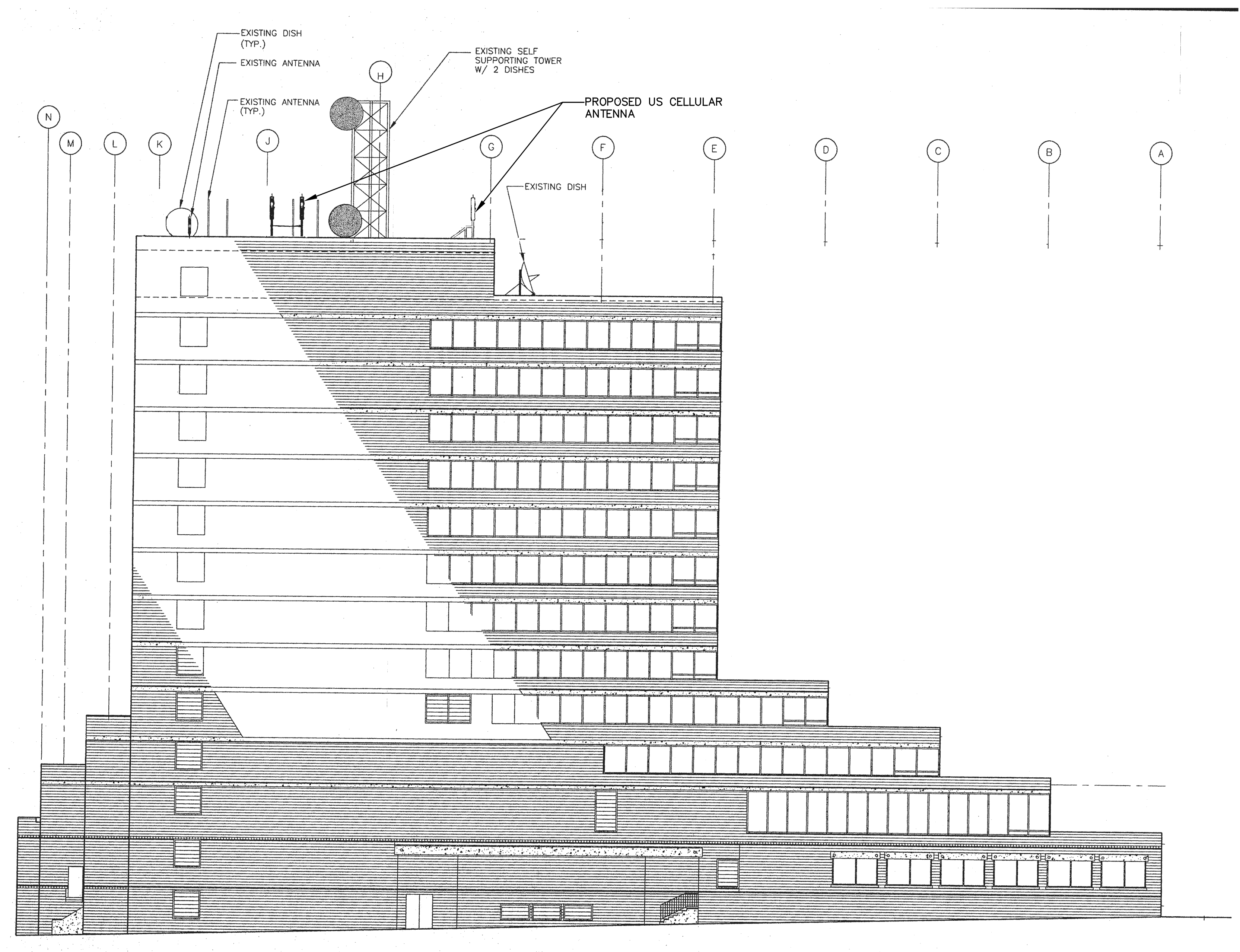
1 FEDERAL STREET (NORTH) ELEVATION E-3 SCALE: 3/4"=1'
