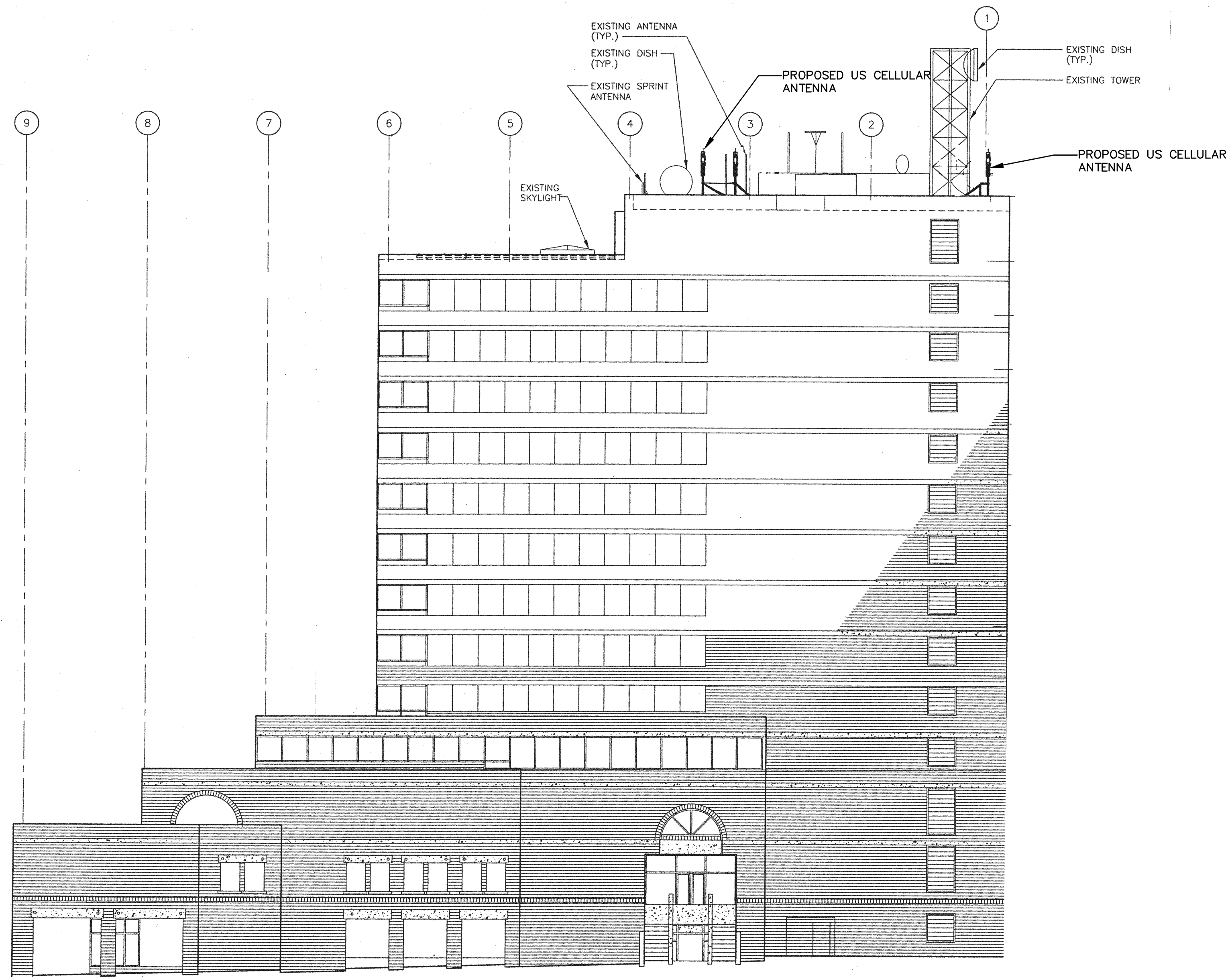
1 TEMPLE STREET (EAST) ELEVATION E-2 SCALE: 3/4"=1'
