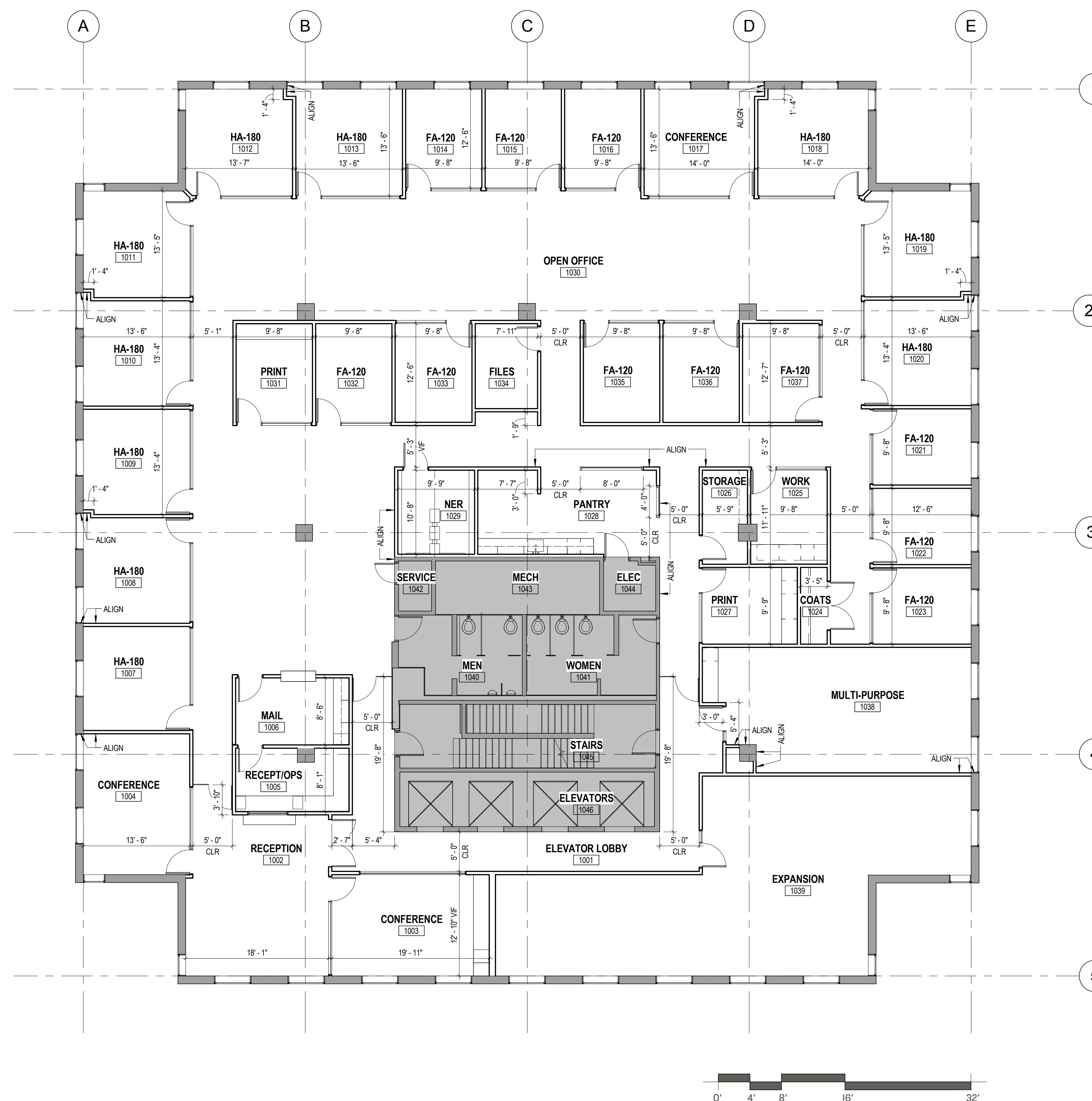
1 10th FLOOR DIMENSION PLAN 1/8" = 1'-0"
