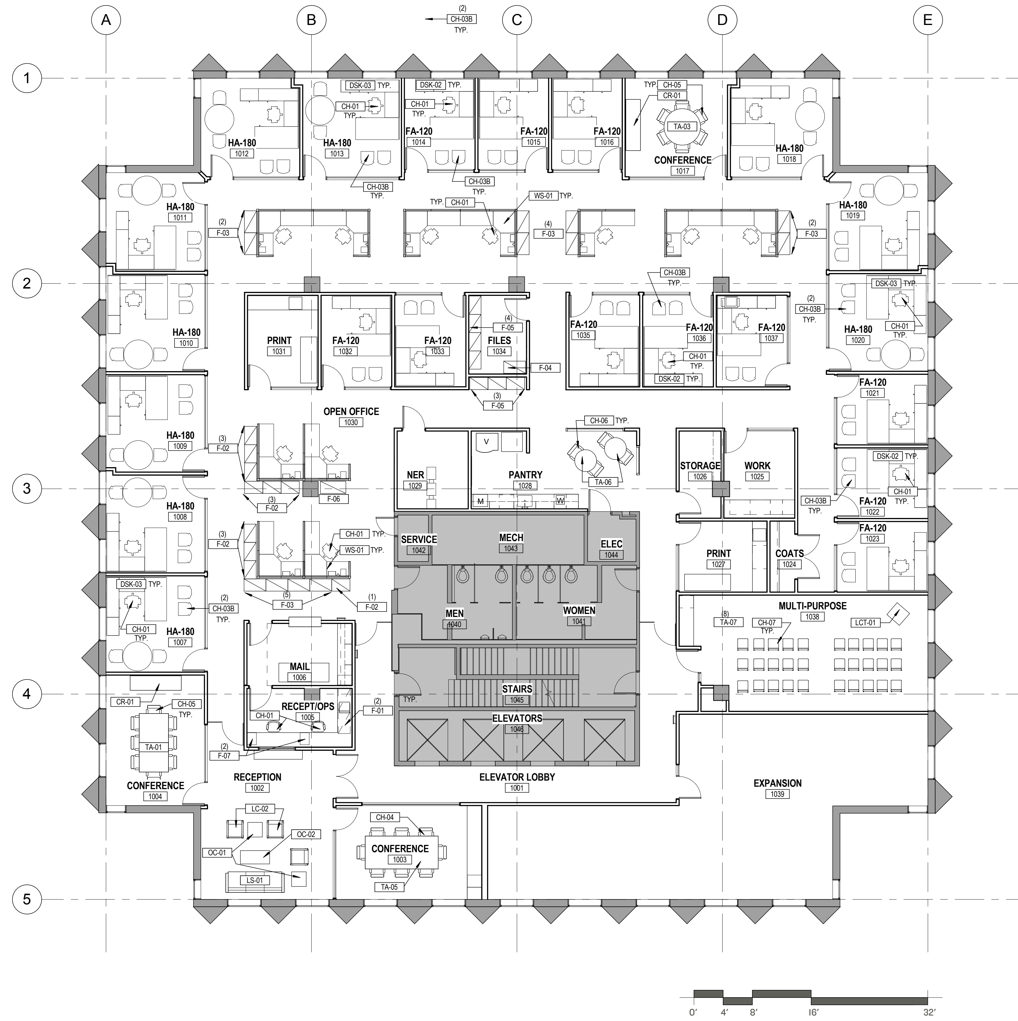
1 10th FLOOR FURNITURE PLAN 1/8" = 1'-0"
